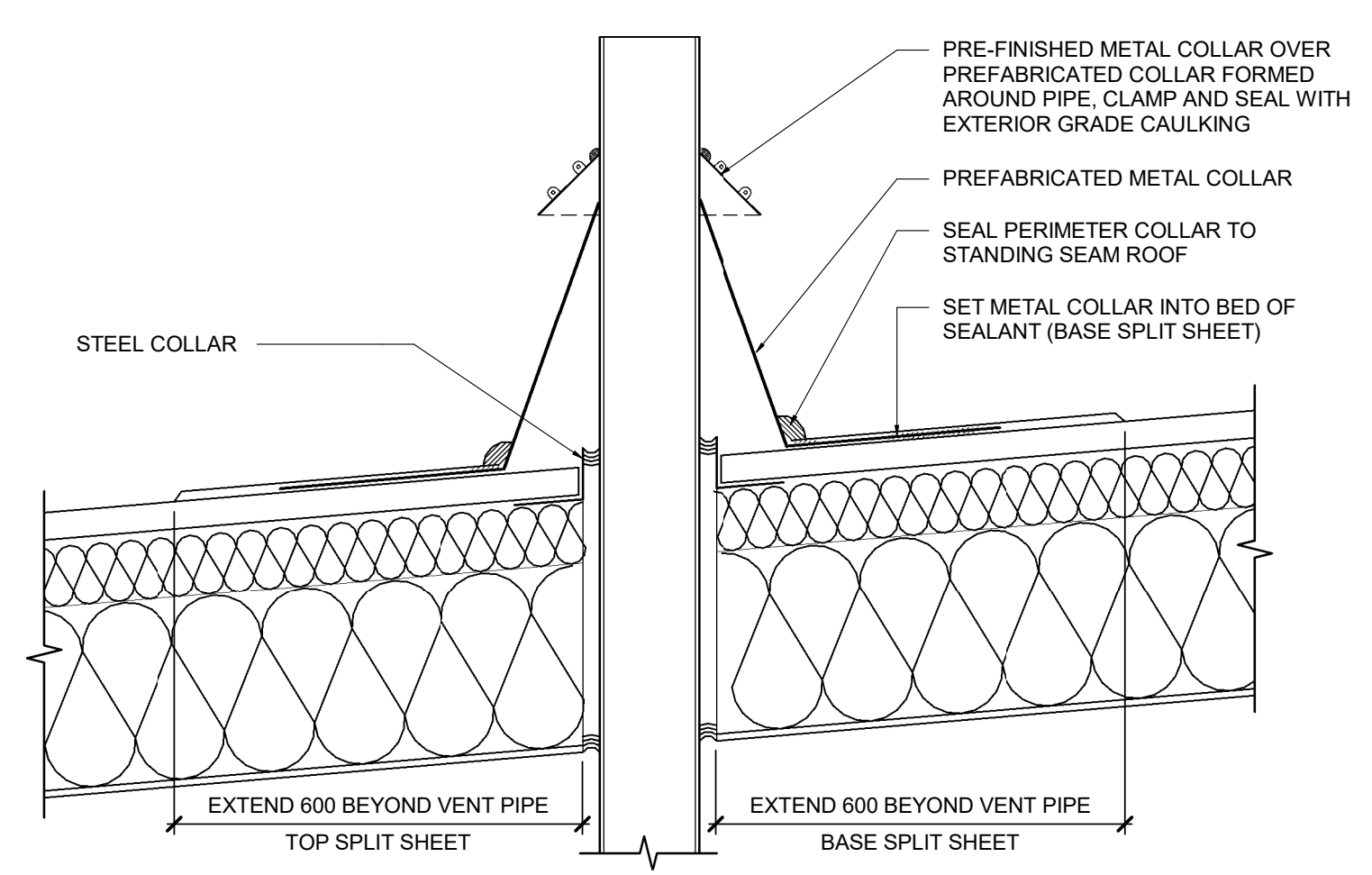
ROOF PIPE PENETRATION DETAIL SCALE: 1:10
