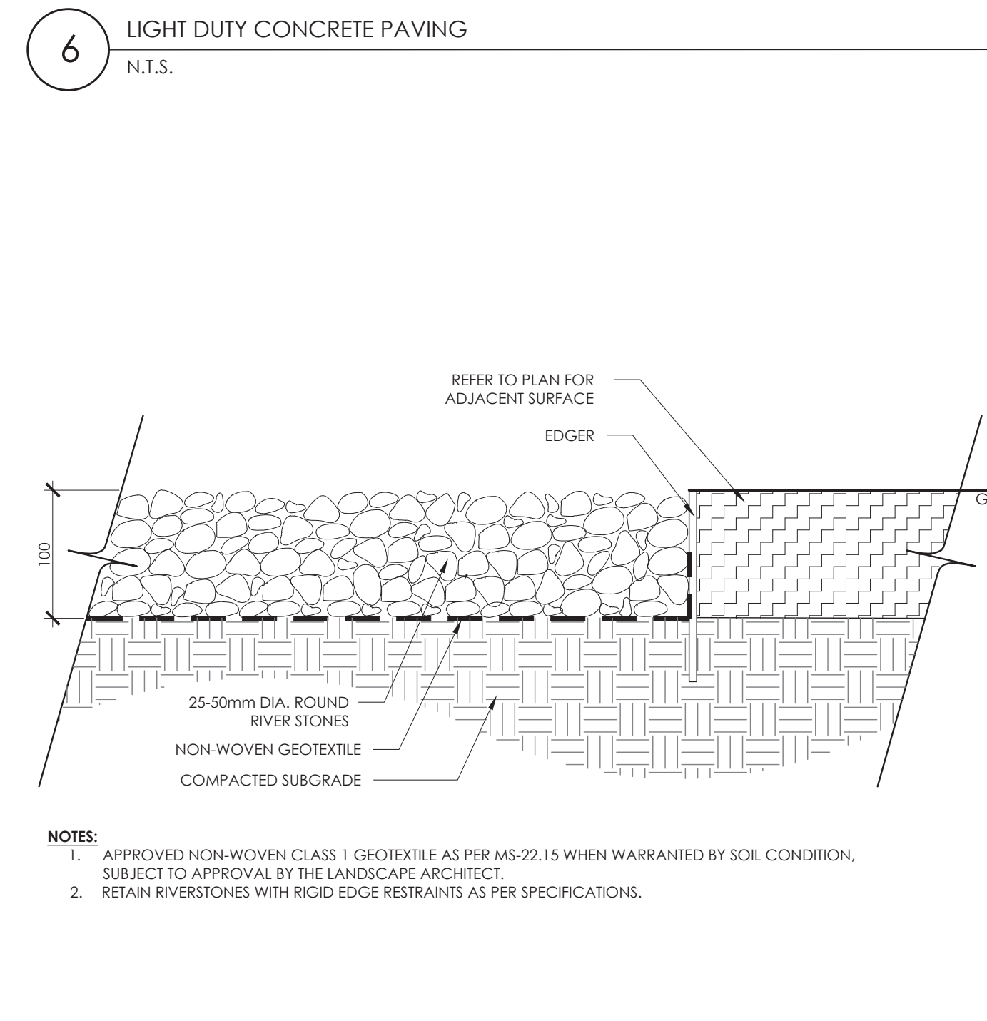
10 RIVER STONE PAVING N.T.S.
