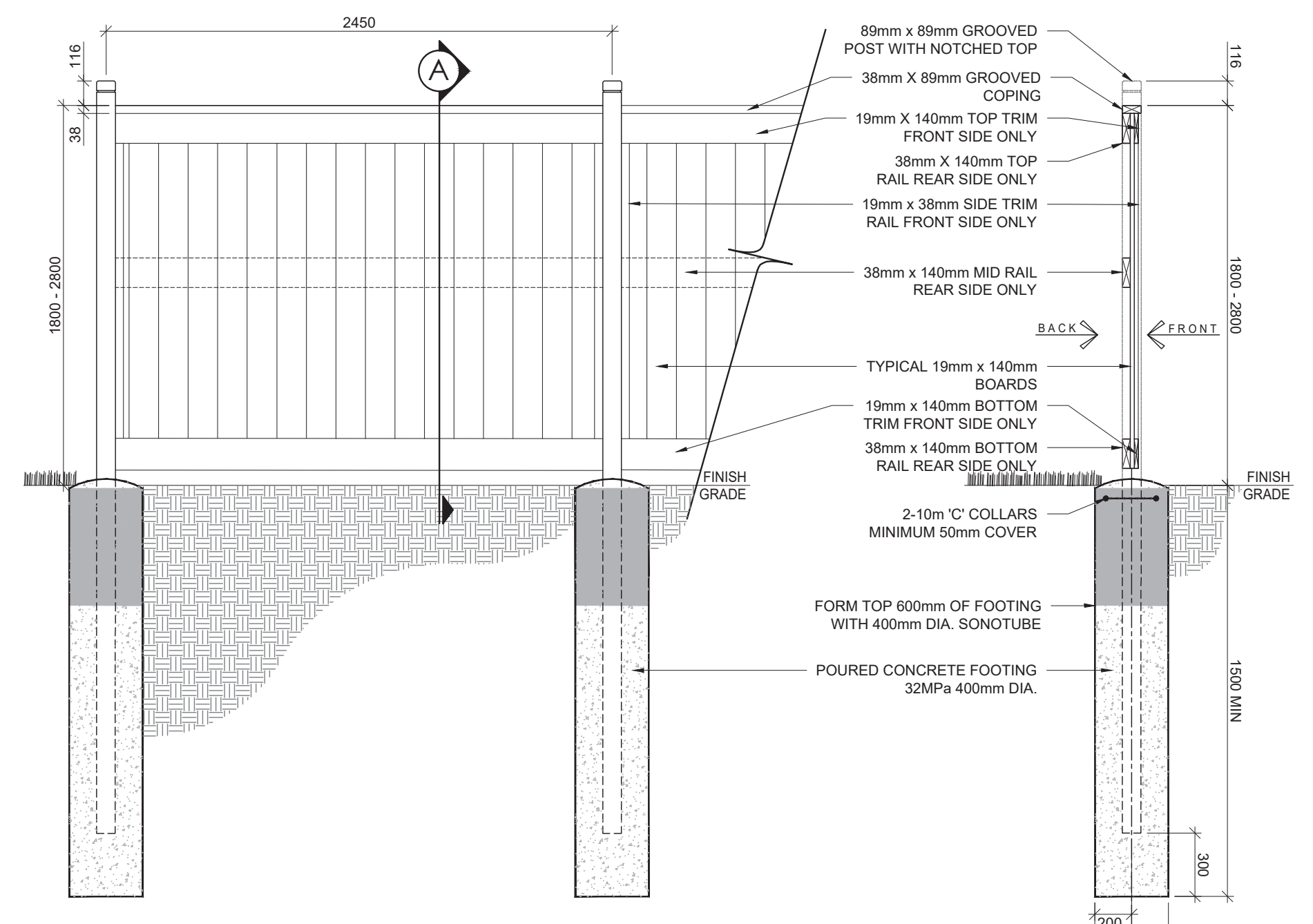
ELEVATION-FRONT SIDE
