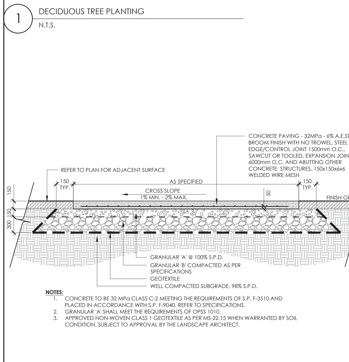
5 HEAVY DUTY CONCRETE PAVING N.T.S.
