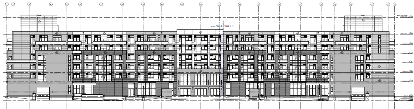
WEST BUILDING KEY ELEVATION SCALE: 1/8" = 1'-0"
