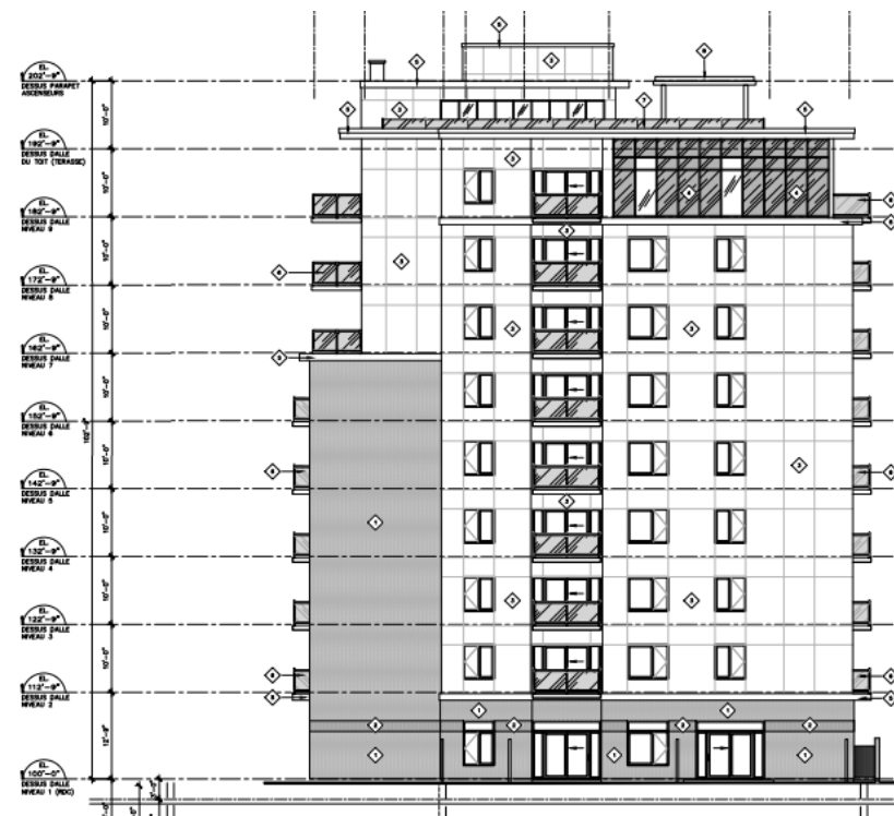
Figure 3: West Elevation of Proposed Development Credit: Caroline Denomme Architects Inc.
