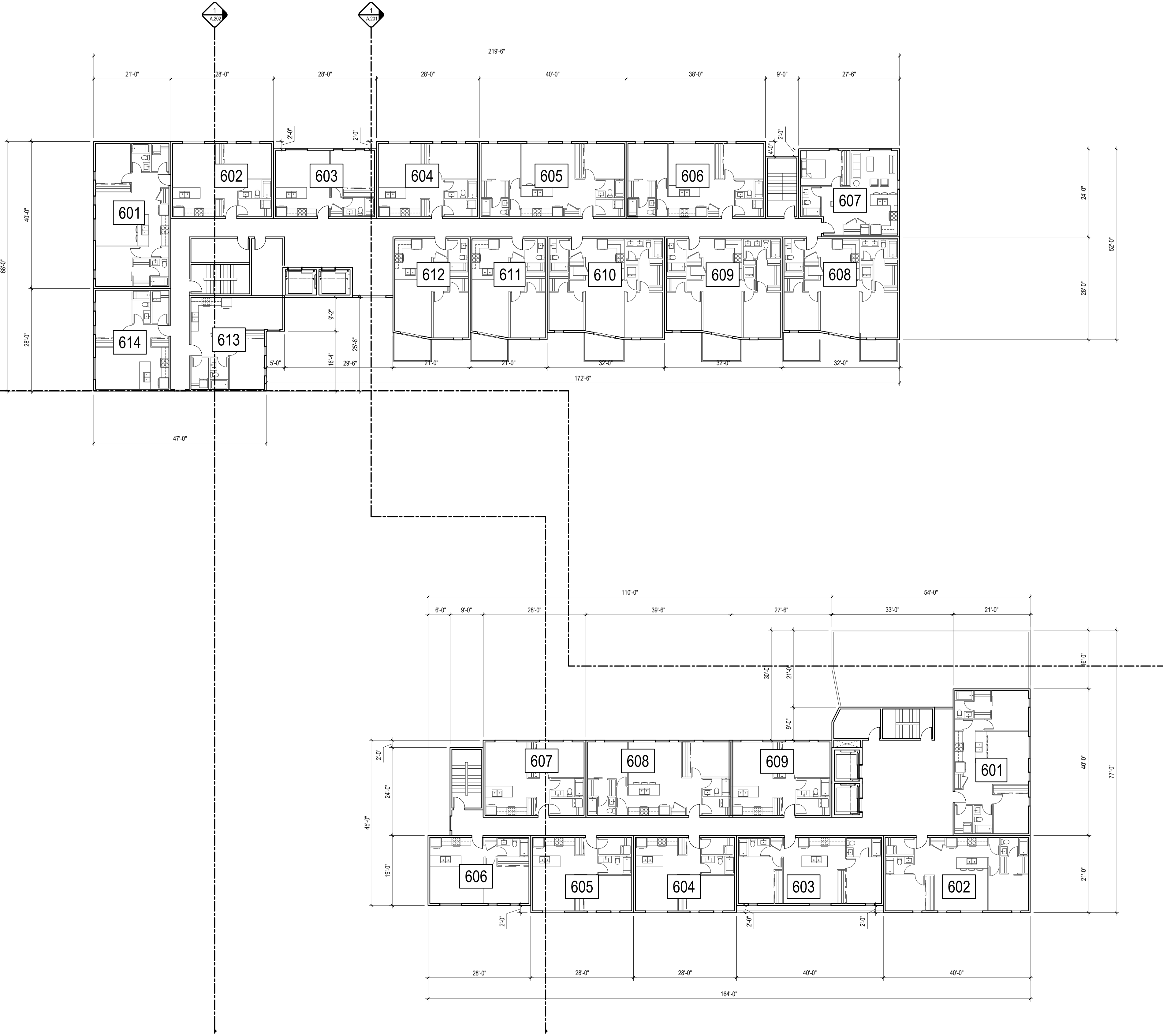
1 LEVEL 06 PLAN DP.106 1/16" = 1'-0"
