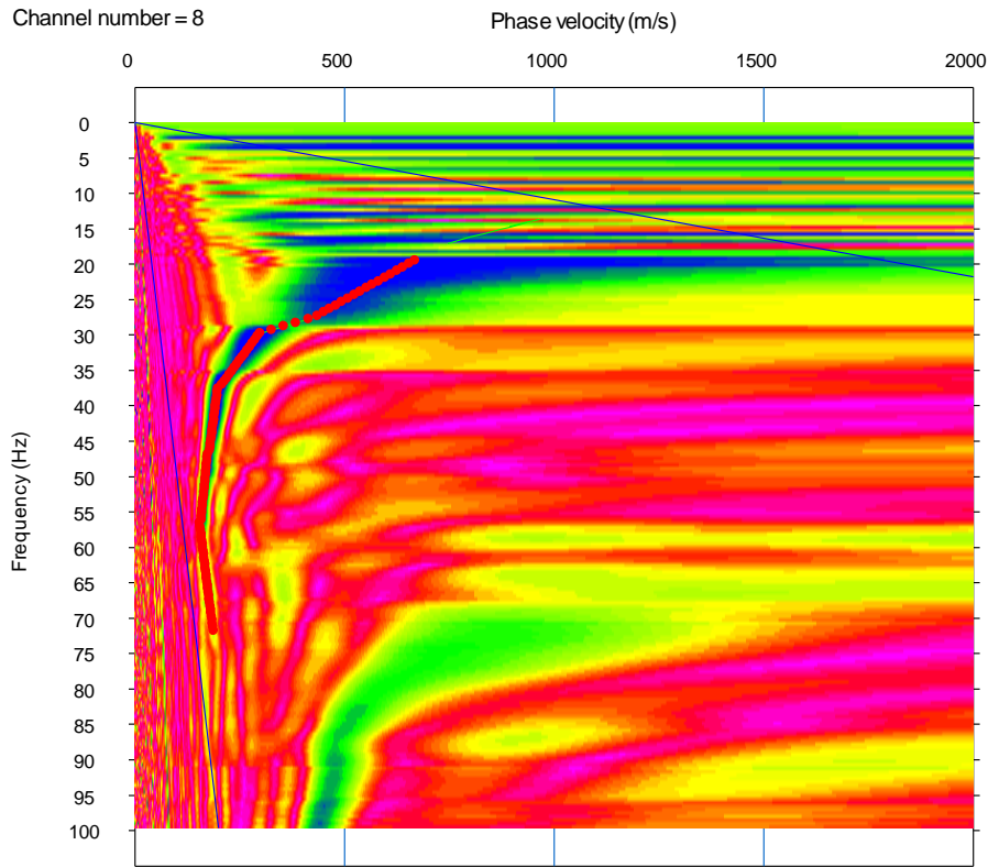
Figure 3: An example dispersion curve.
