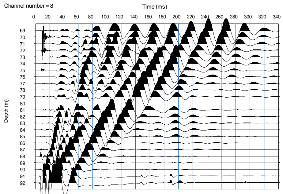
Figure 2: An example shot record.
