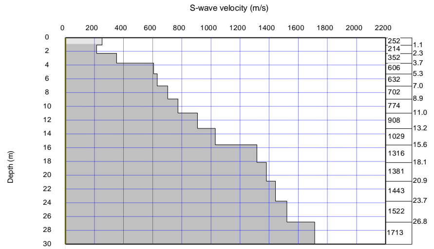
Figure 4: Resulting 1-D V_s profile. Average V_{s30} value is approximately 688 m/s.
