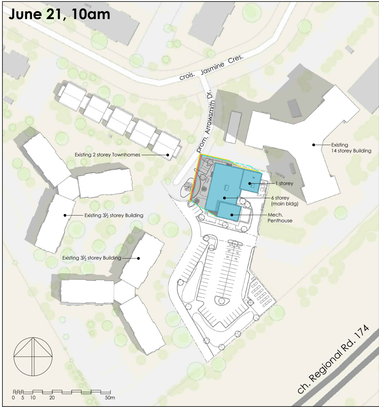
2040 ARROWSMITH - TOP VIEW SHADOW STUDY FIGURE: TEST TIME - JUNE 21 at 10am / 11am (UTC-05:00)
