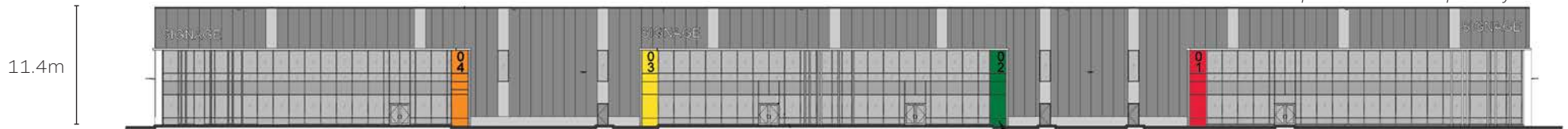
North Elevation
