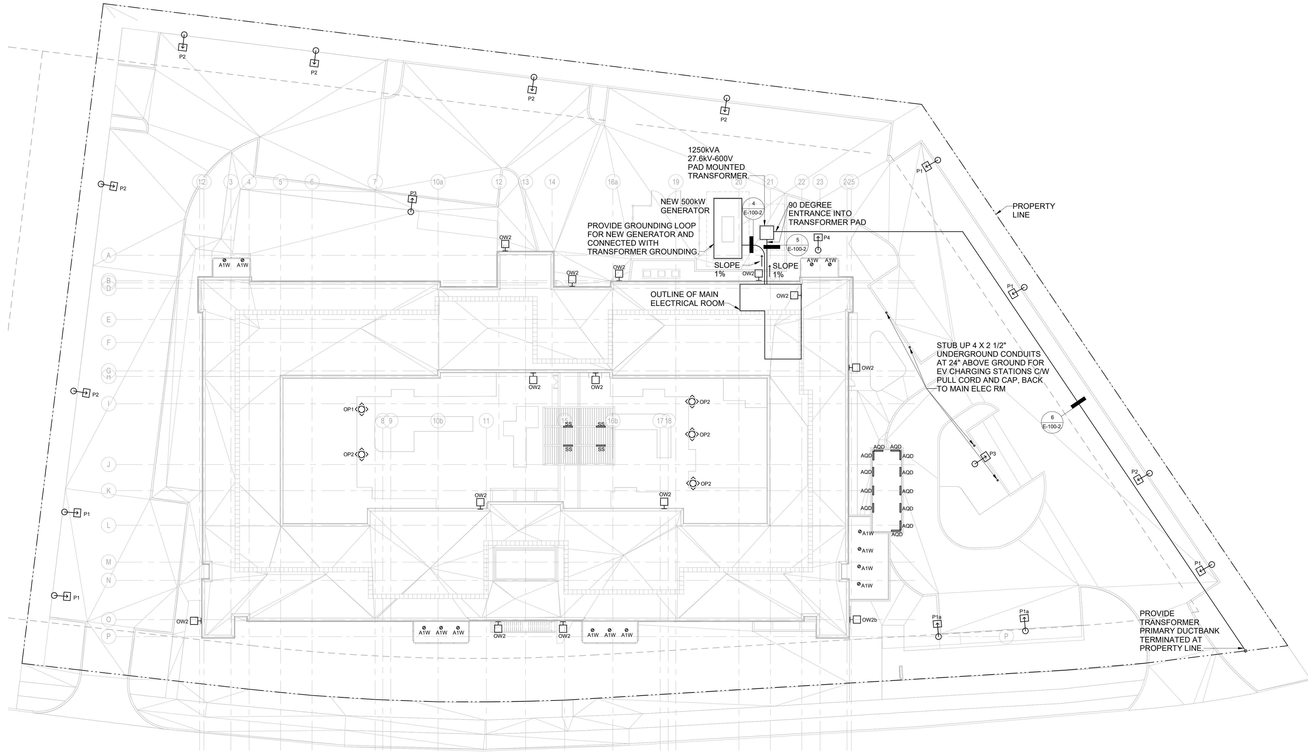
1 ELECTRICAL SITE PLAN - POWER & SYSTEMS. SCALE: 1 : 250
