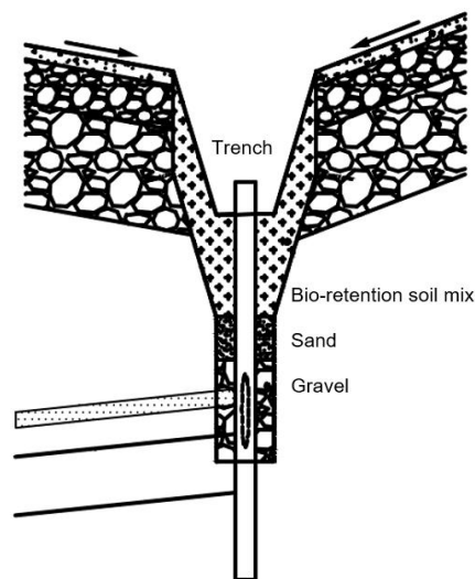
Figure 2: Bioswale cross-section
