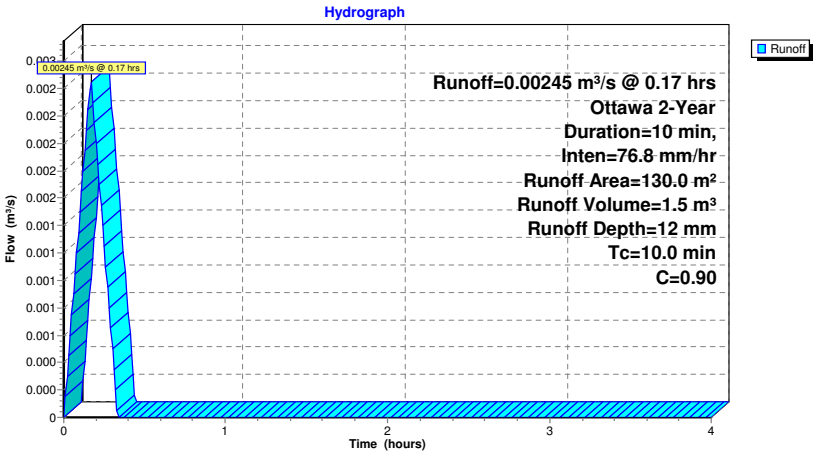
Subcatchment 10S: B-102
