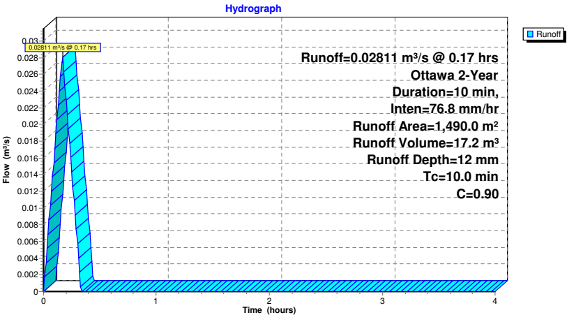
Subcatchment 11S: BLDG1 Roof
