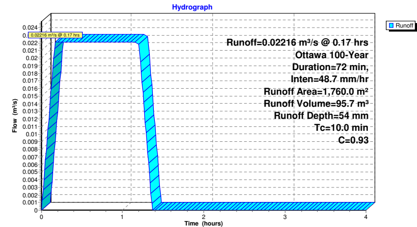
Subcatchment A-103: Proposed to Ditch
