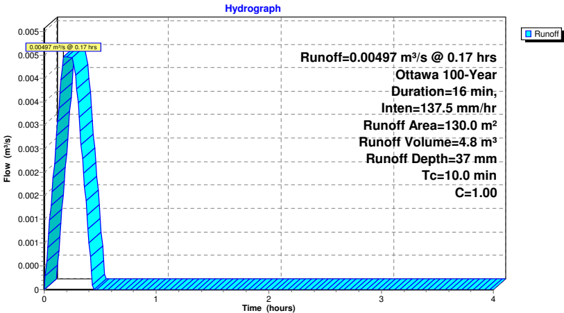
Subcatchment B-102: B-102
