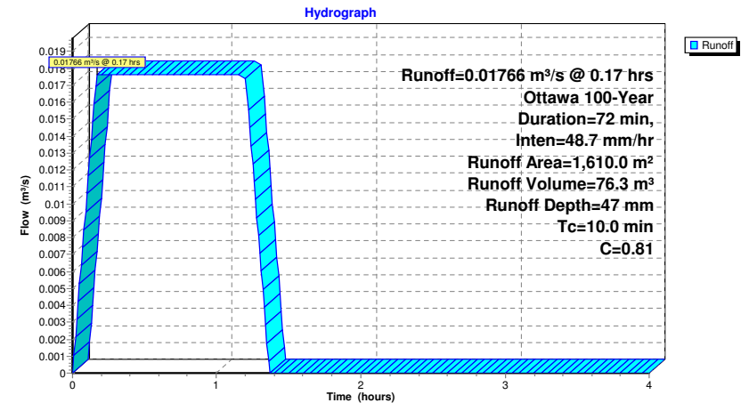
Subcatchment B-101: B-101
