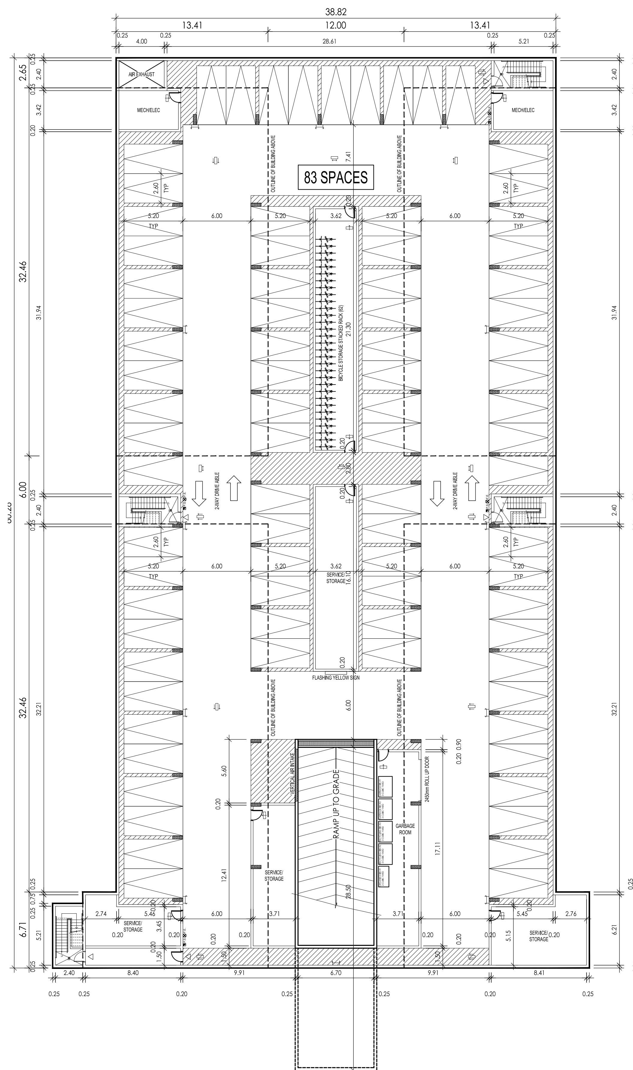
1 SOUTH GARAGE (MT-4 to MT-7) 1:200
