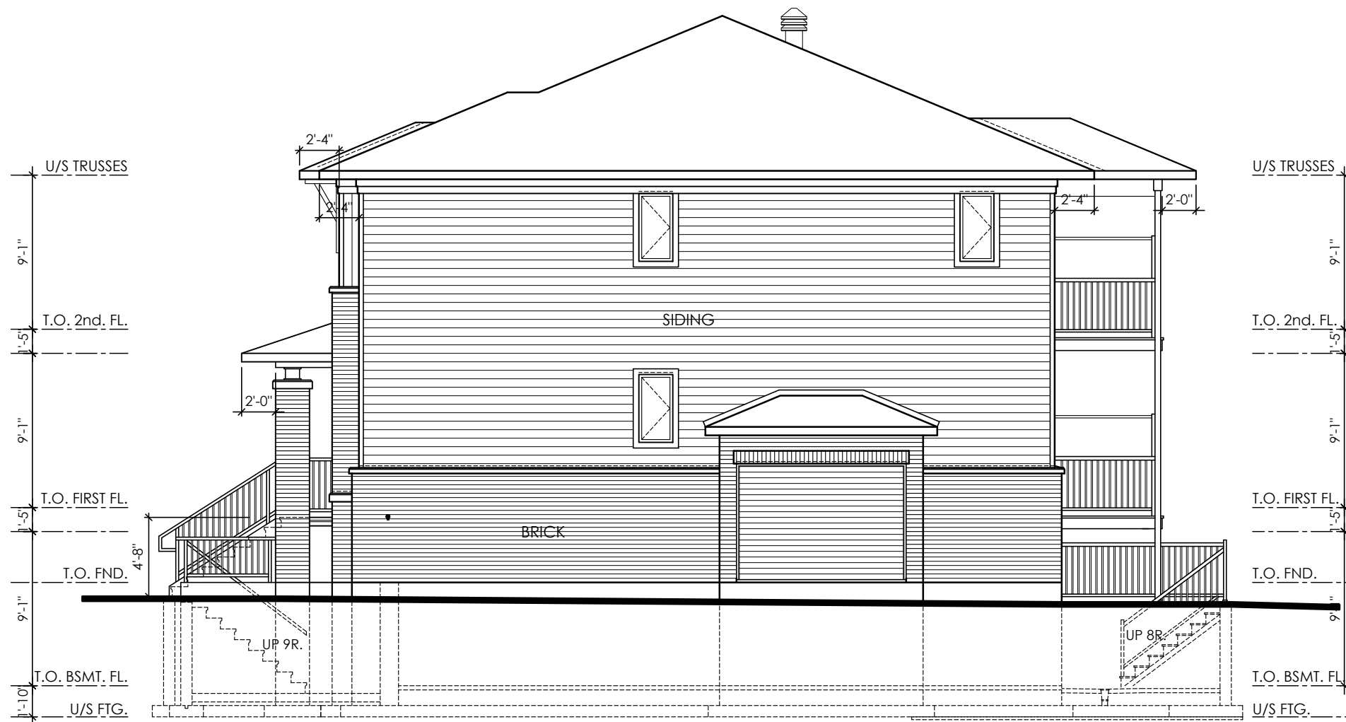
END UNIT REV. END UNIT, SIDE ELEVATION
