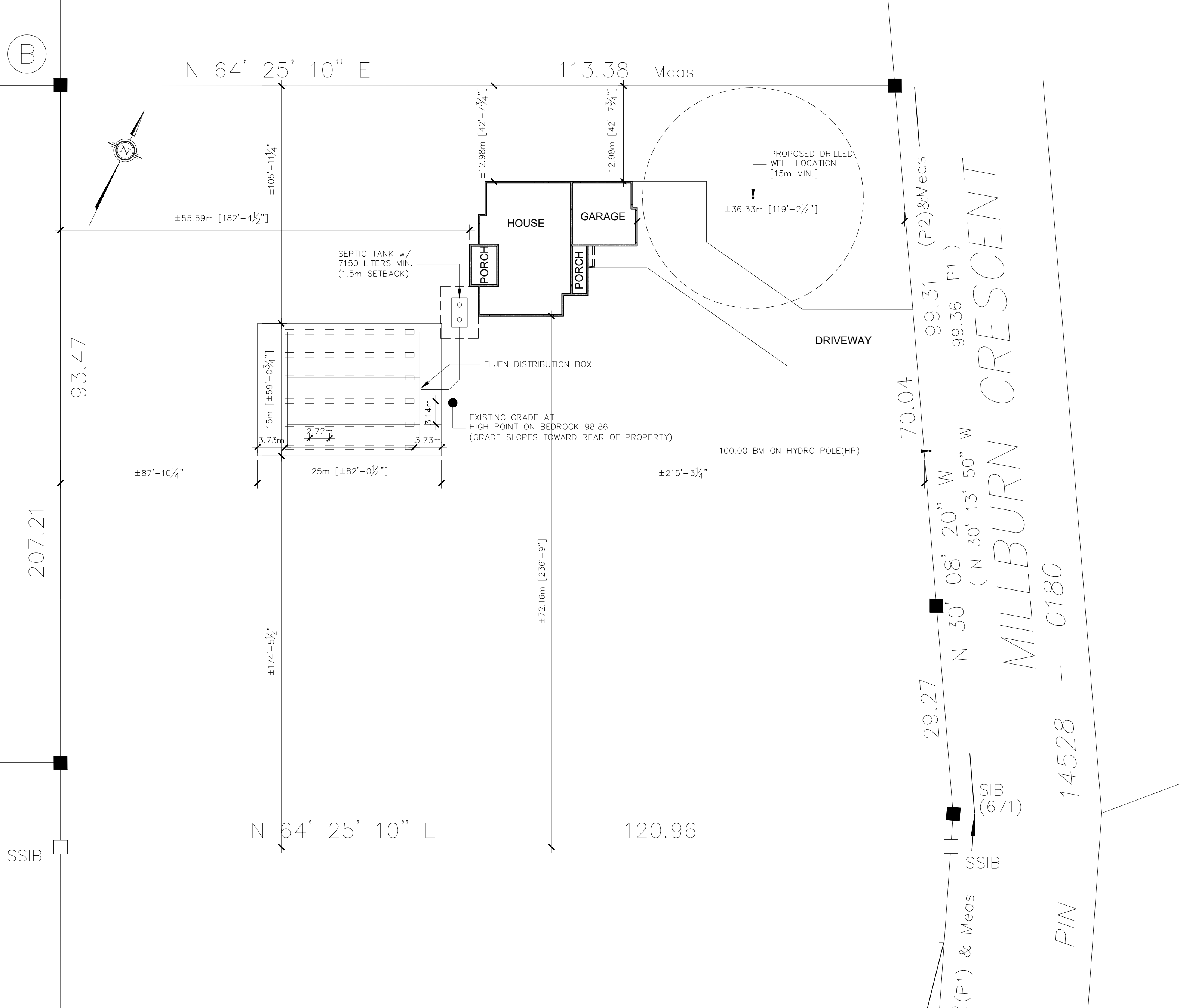
PROPOSED - SITE PLAN + SEPTIC DESIGN LOCATION
