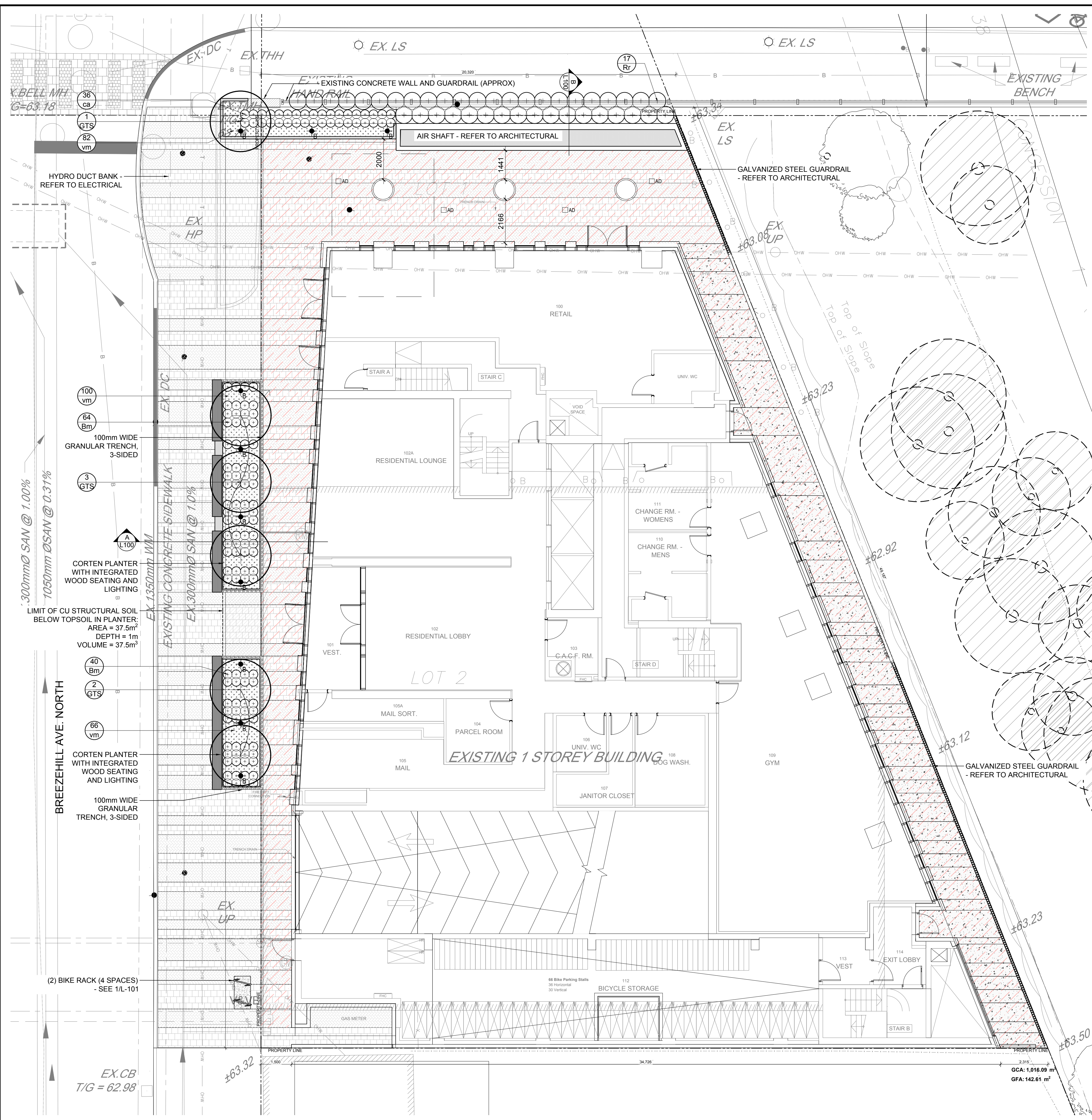
1 LANDSCAPE PLAN - GROUND FLOOR SCALE 1:100
