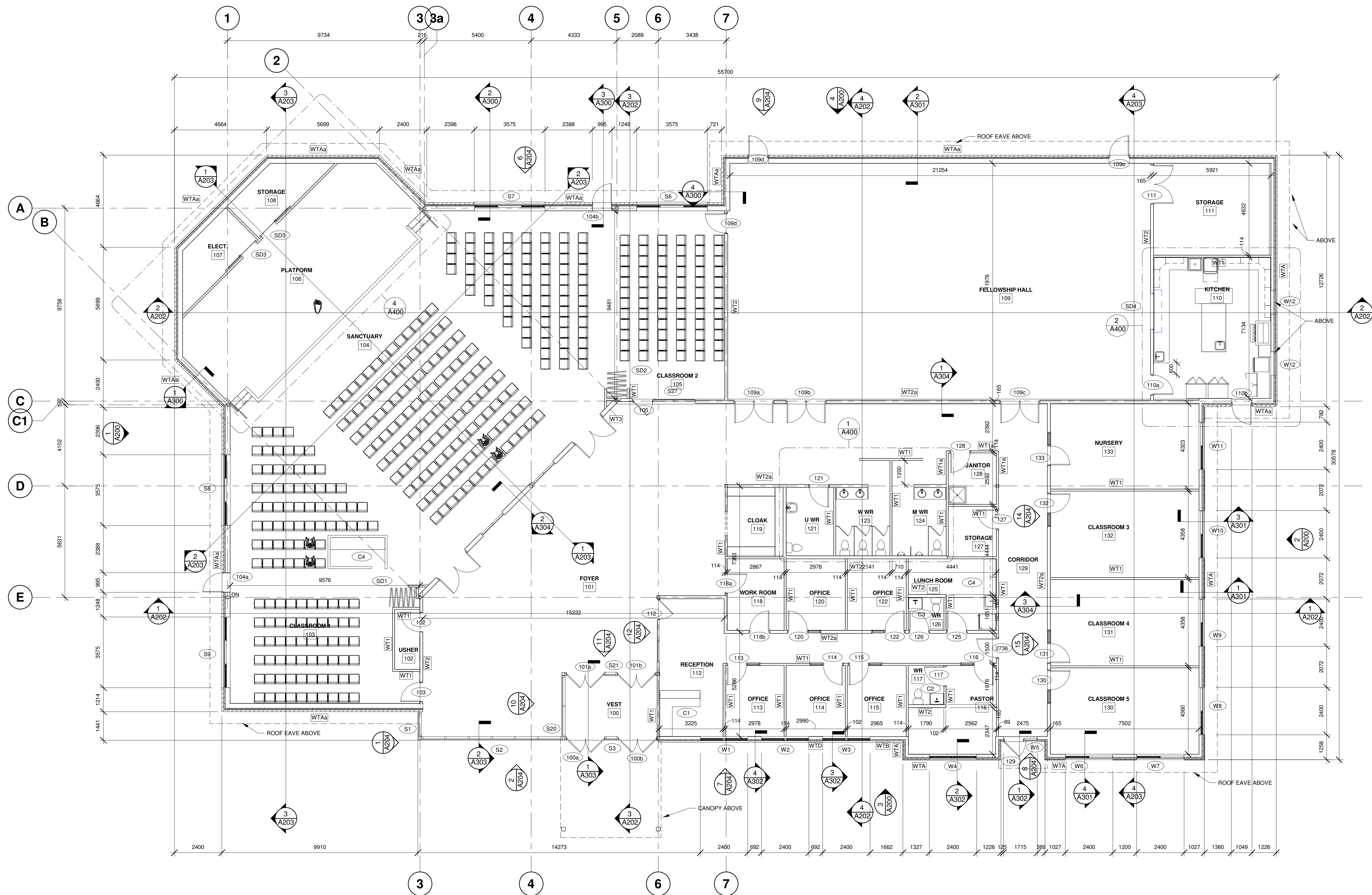
1 MAIN LEVEL FLOOR PLAN 1 : 100
