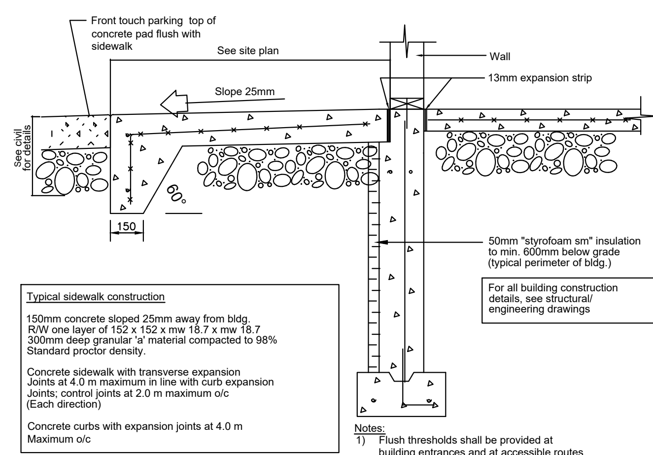
TYPICAL SIDEWALK DETAIL section NTS
