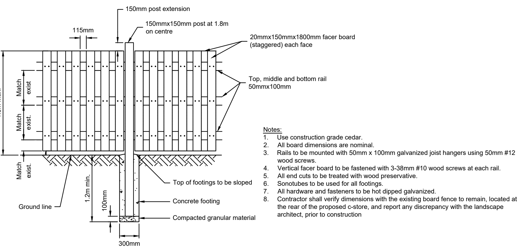
SHADOWBOX WOOD FENCE section NTS
