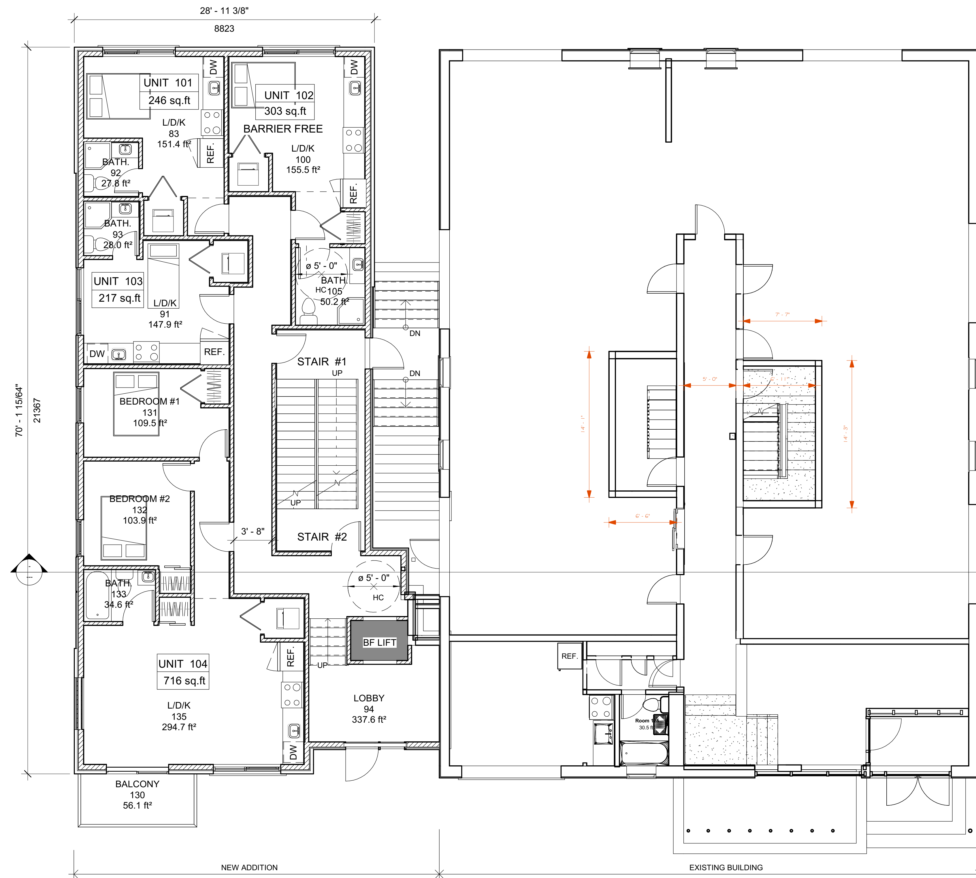
1 Ground Floor 3/16" = 1'-0"
