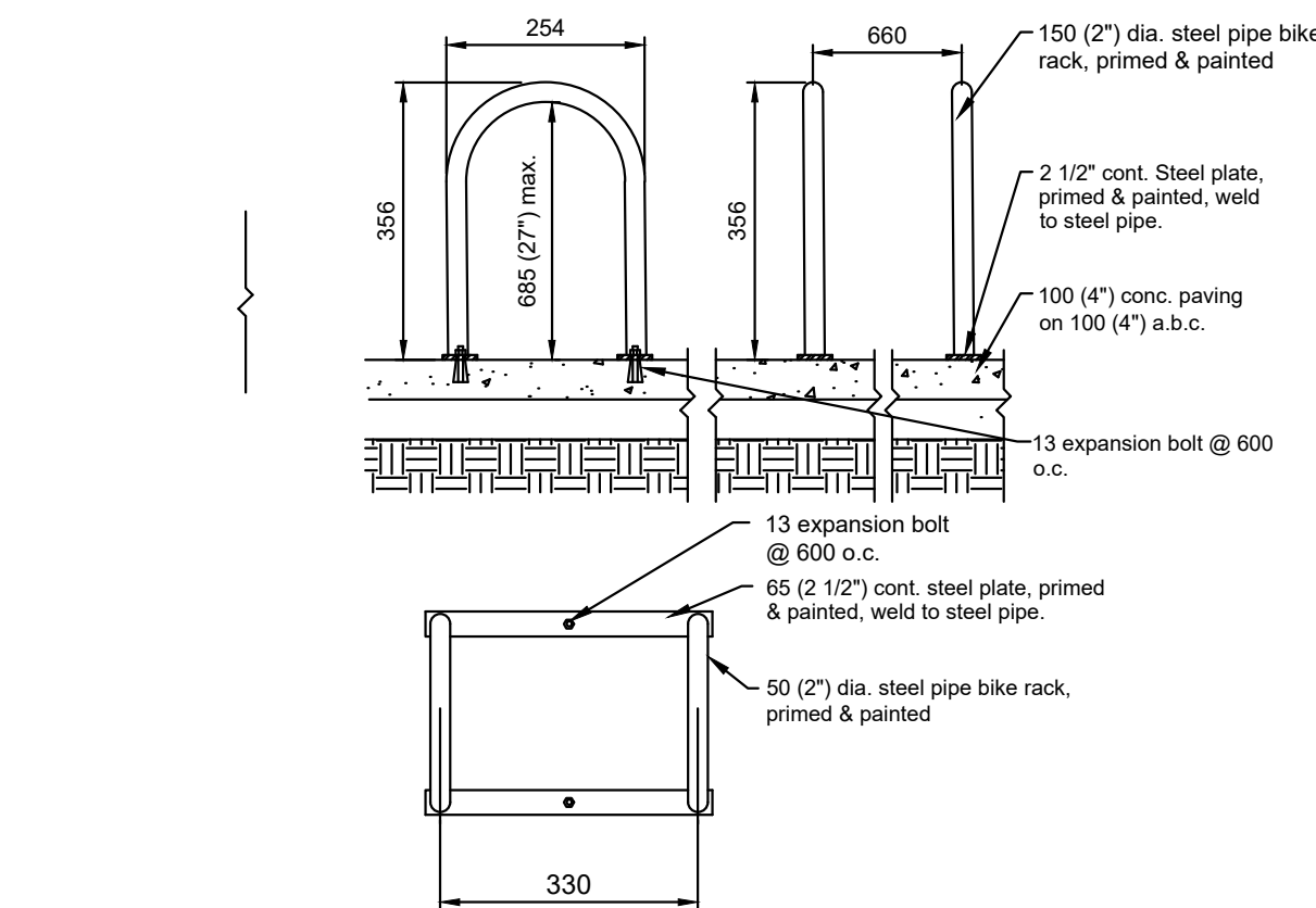
BIKE RACK section NTS
