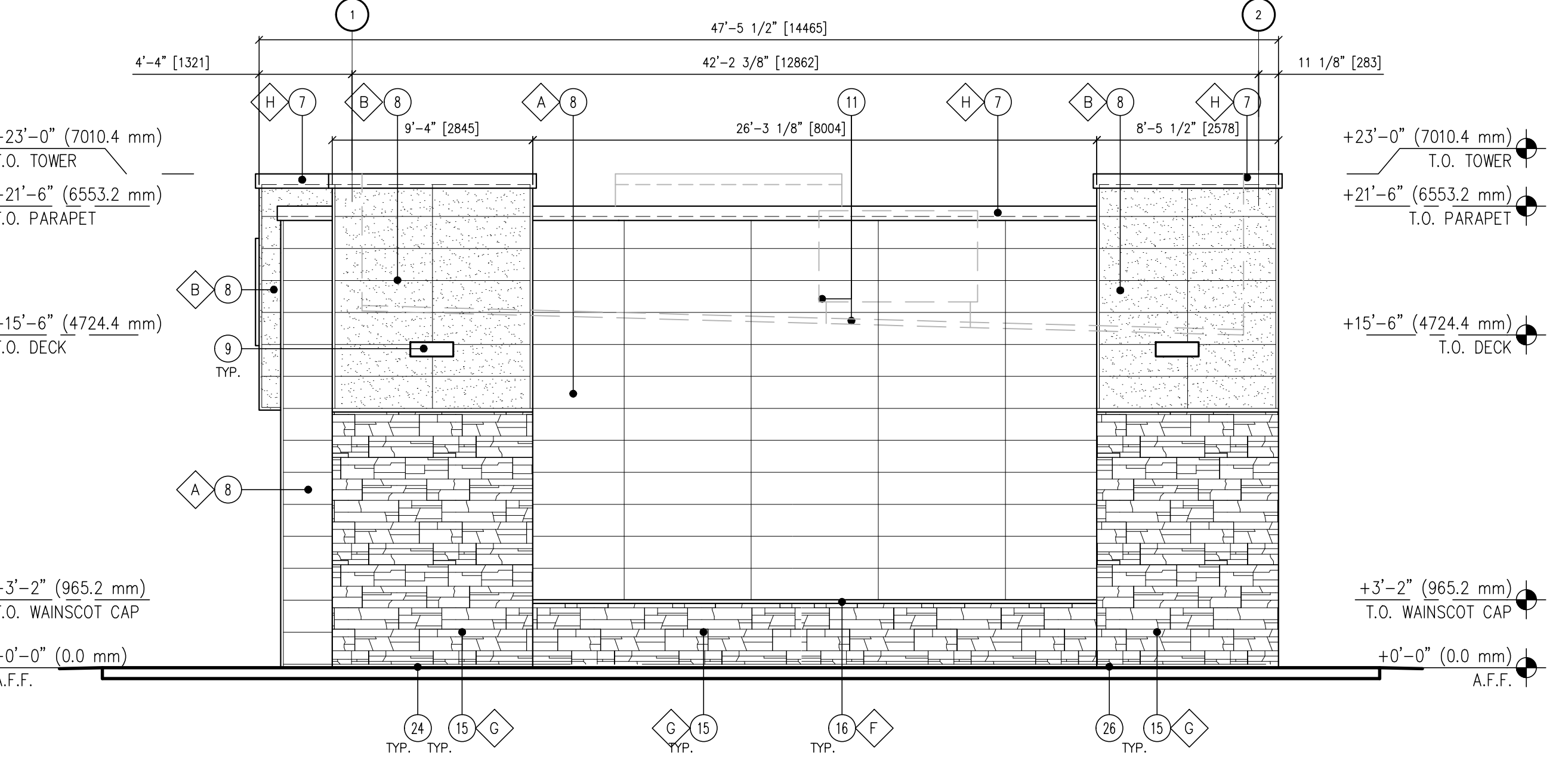
3 SIDE (SOUTH) ELEVATION SCALE: 3/16" = 1'-0"
