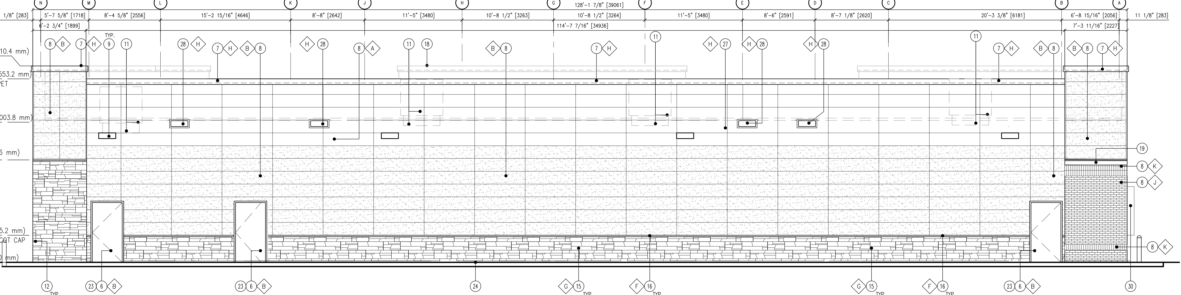
2 BACK (EAST) ELEVATION SCALE: 3/16" = 1'-0"
