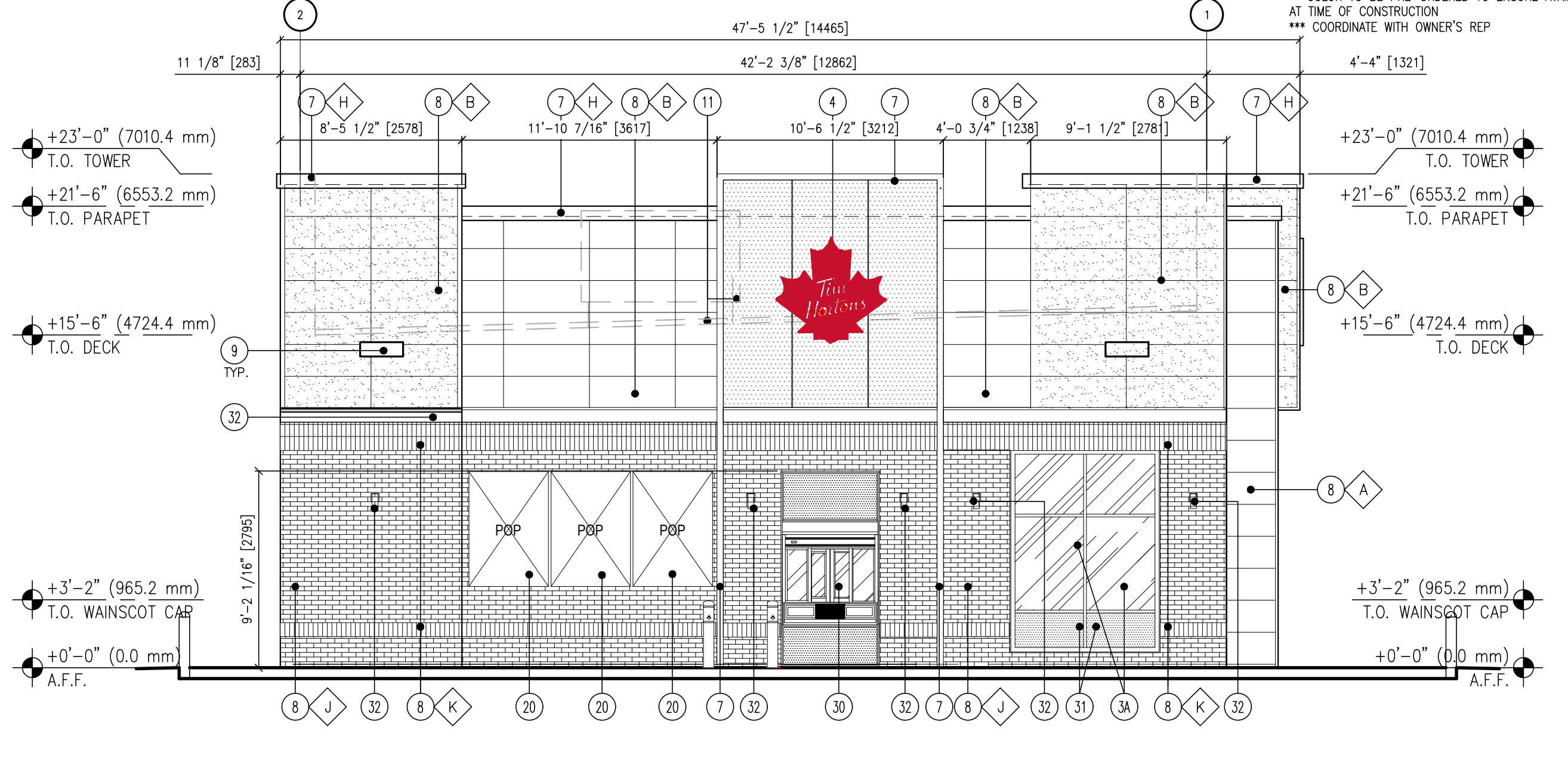
4 SIDE (NORTH) ELEVATION SCALE: 3/16" = 1'-0"
