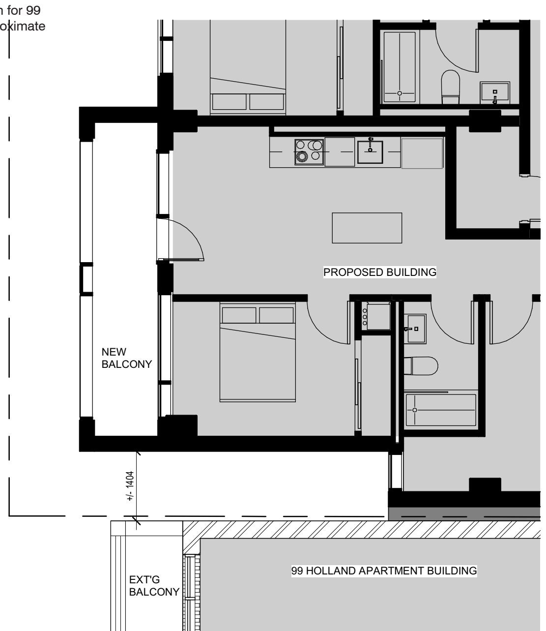
2 FLOOR PLAN - BALCONY RELATIONSHIP WITH 99 HOLLAND
