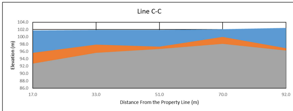
Figure 6-6: Cross-section C-C
