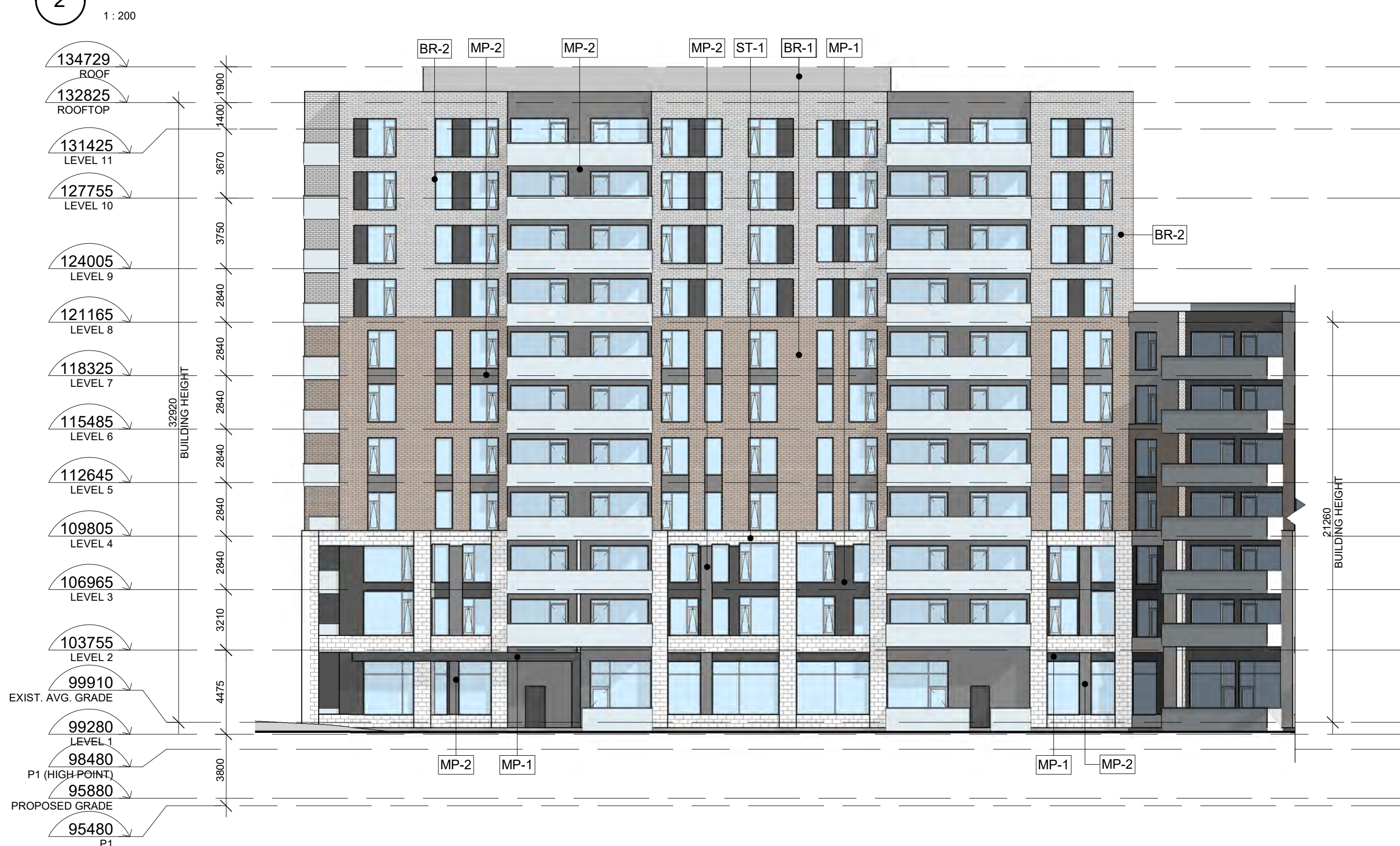
3 NORTH ELEVATION - EAST BUILDING
