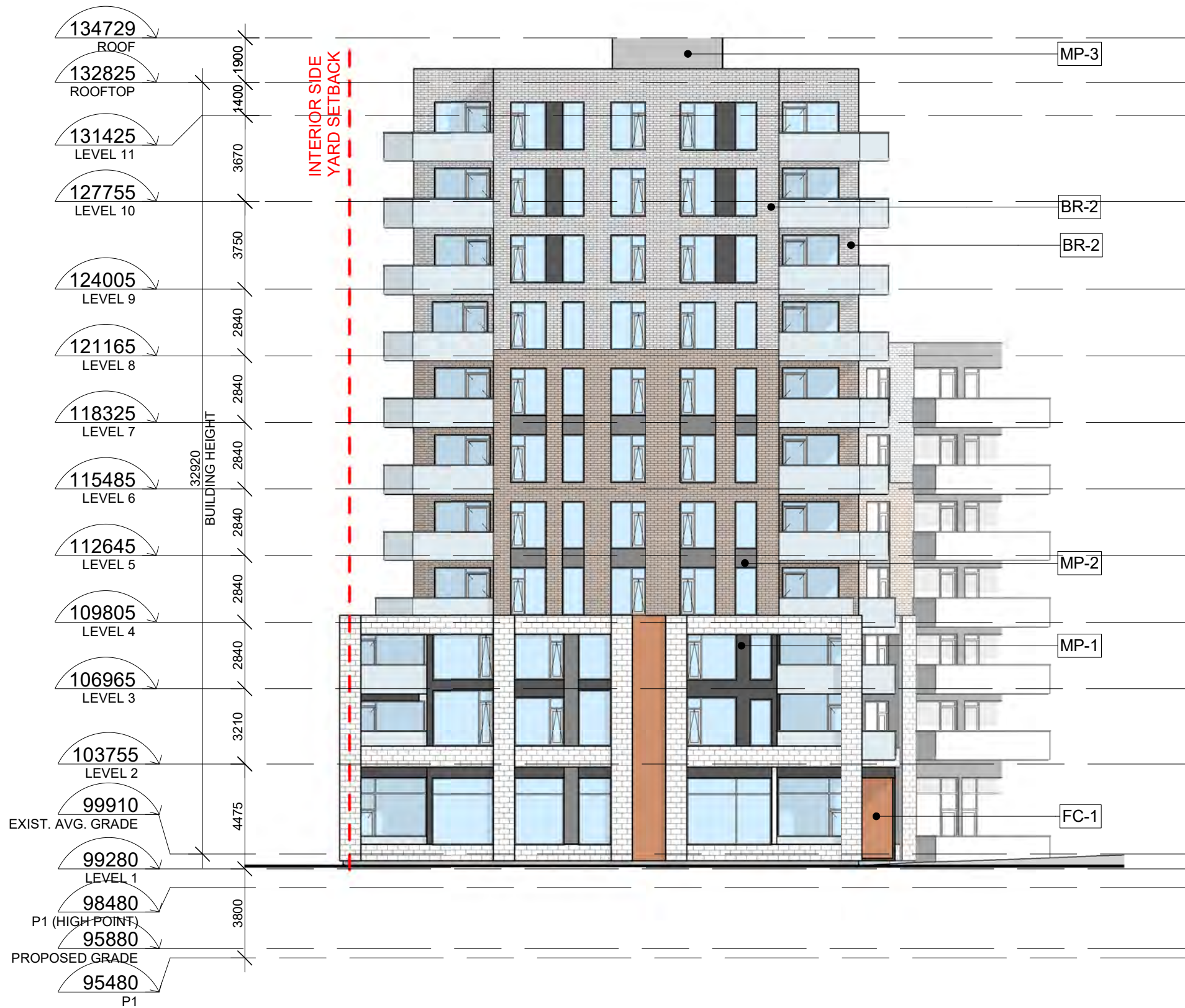
4 EAST ELEVATION
