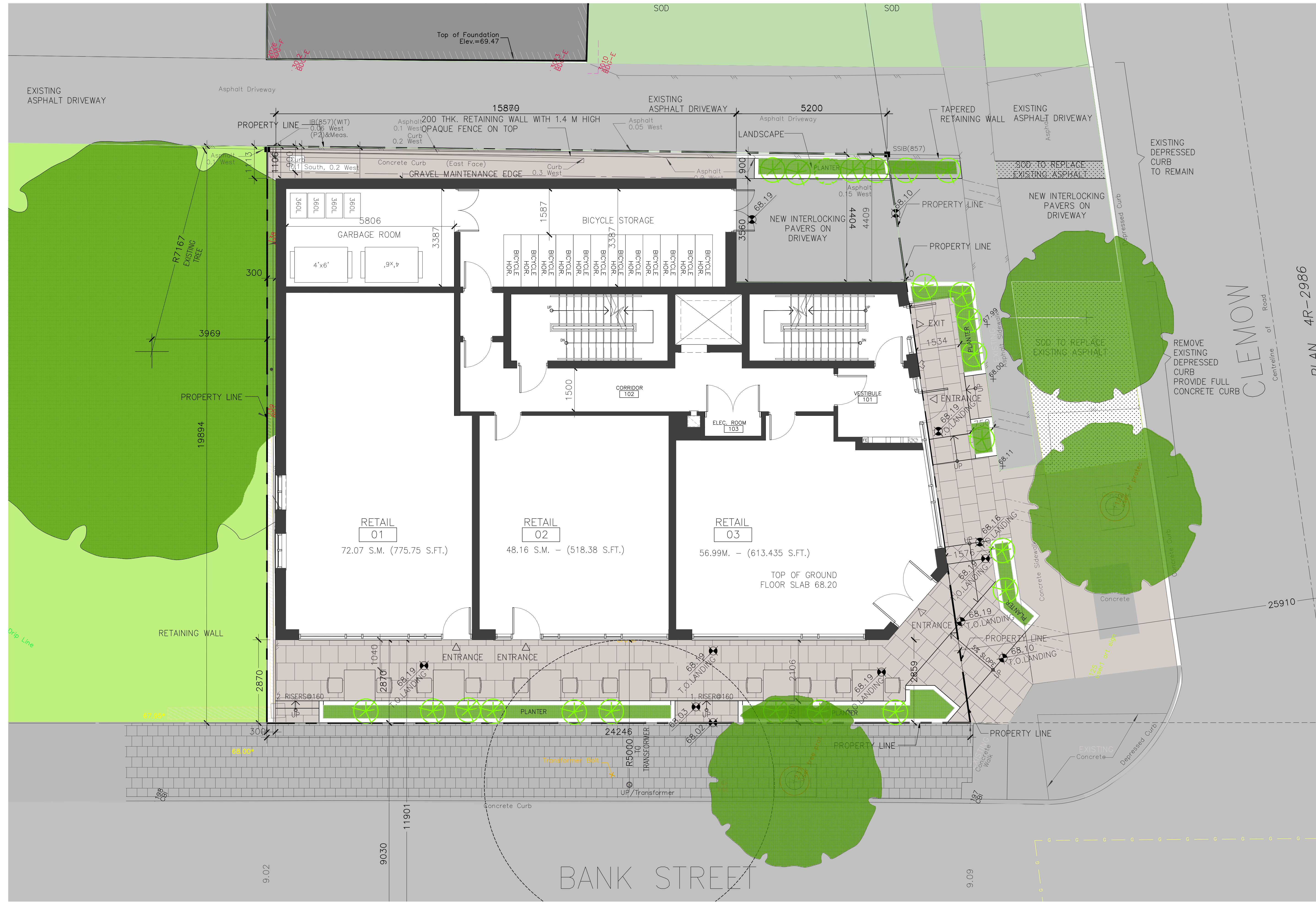
1 A1.1 GROUND FLOOR PLAN SCALE 1:50
