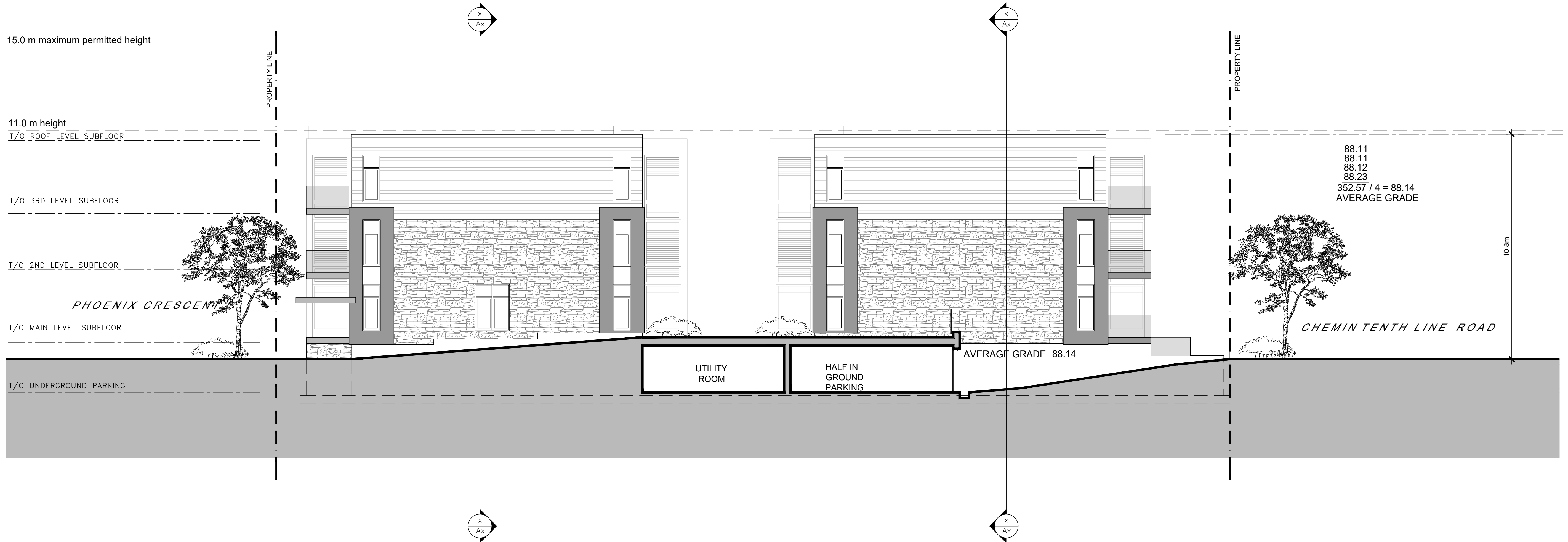
2 SOUTH SIDE ELEVATION A-200 SCALE = 1:100
