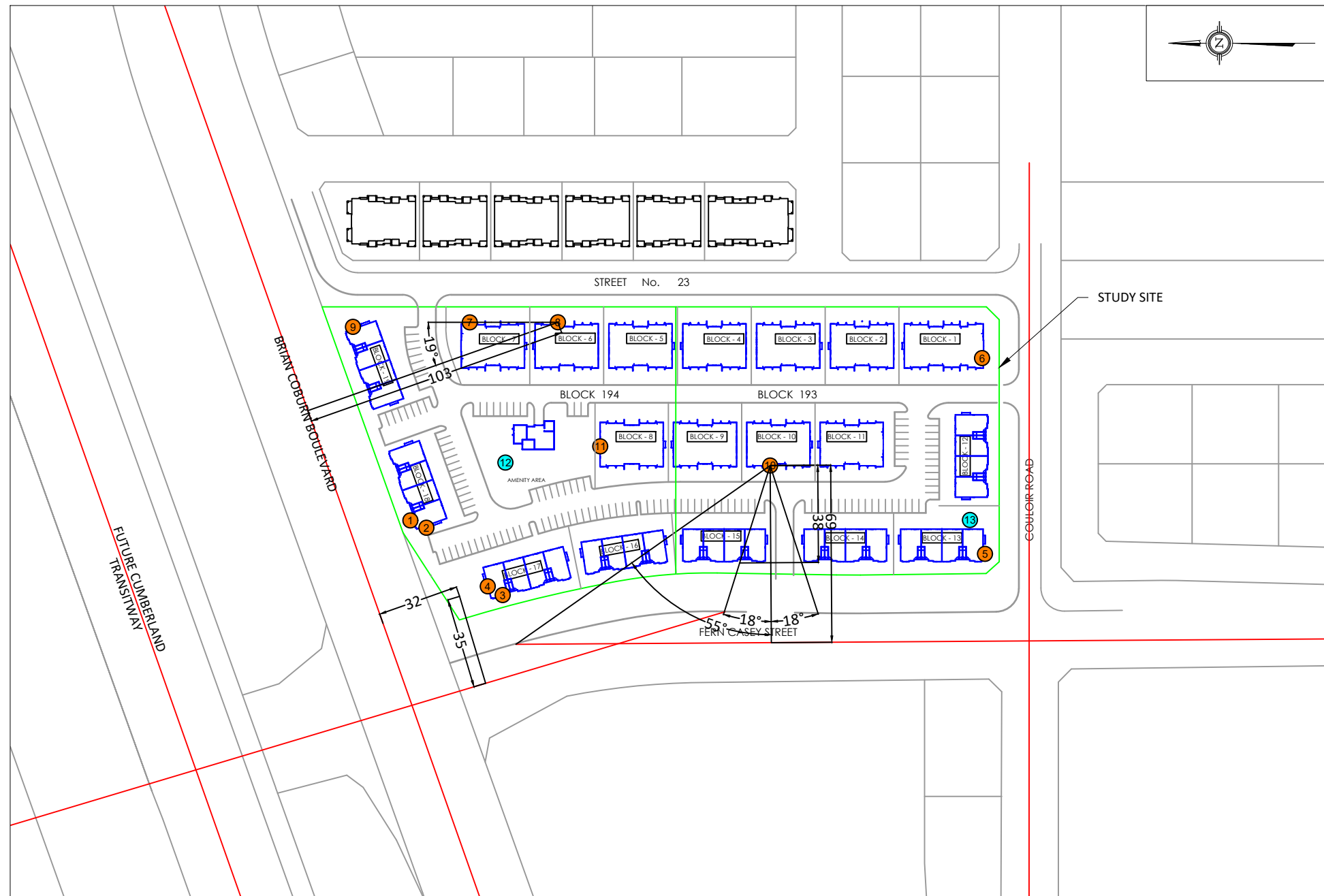
DESCRIPTION FIGURE 7: STAMSON INPUT PARAMETERS - RECEPTOR 4,8,10
