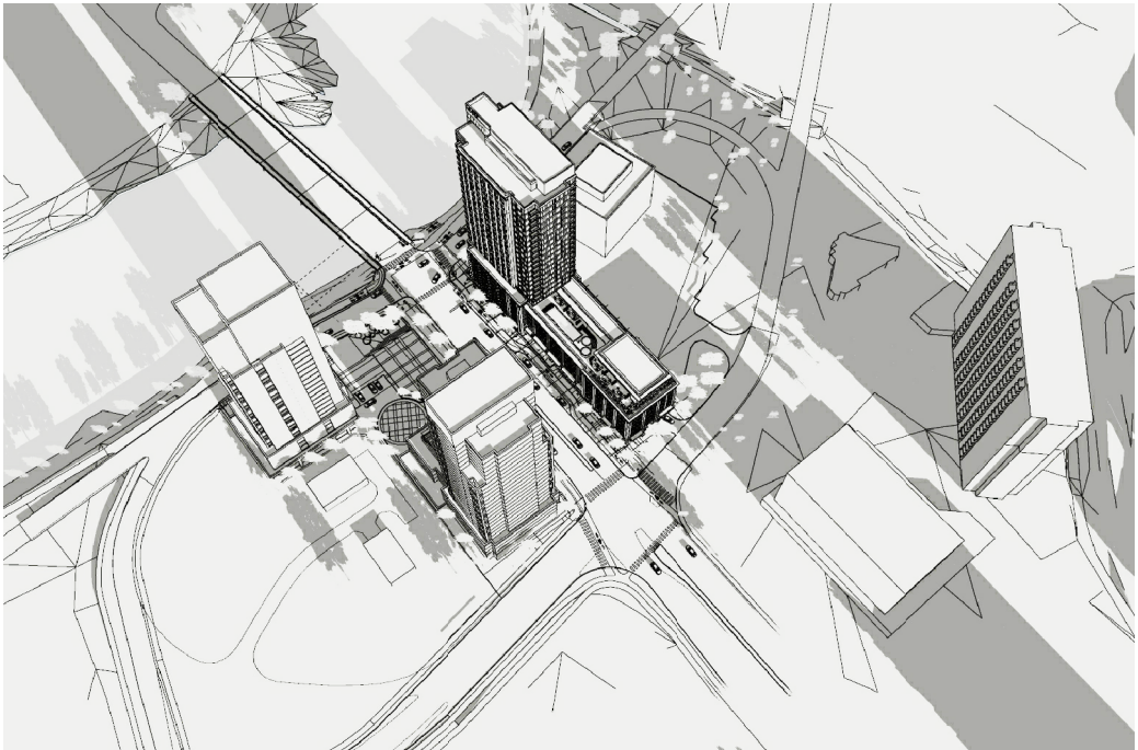
DEC 21 - 10AM
