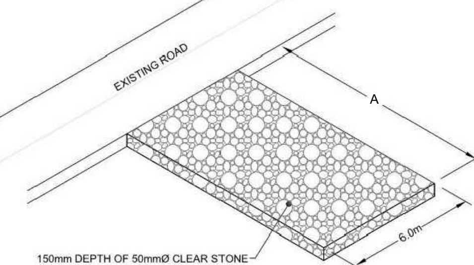
MUD MAT - CONSTRUCTION ACCESS NTS
