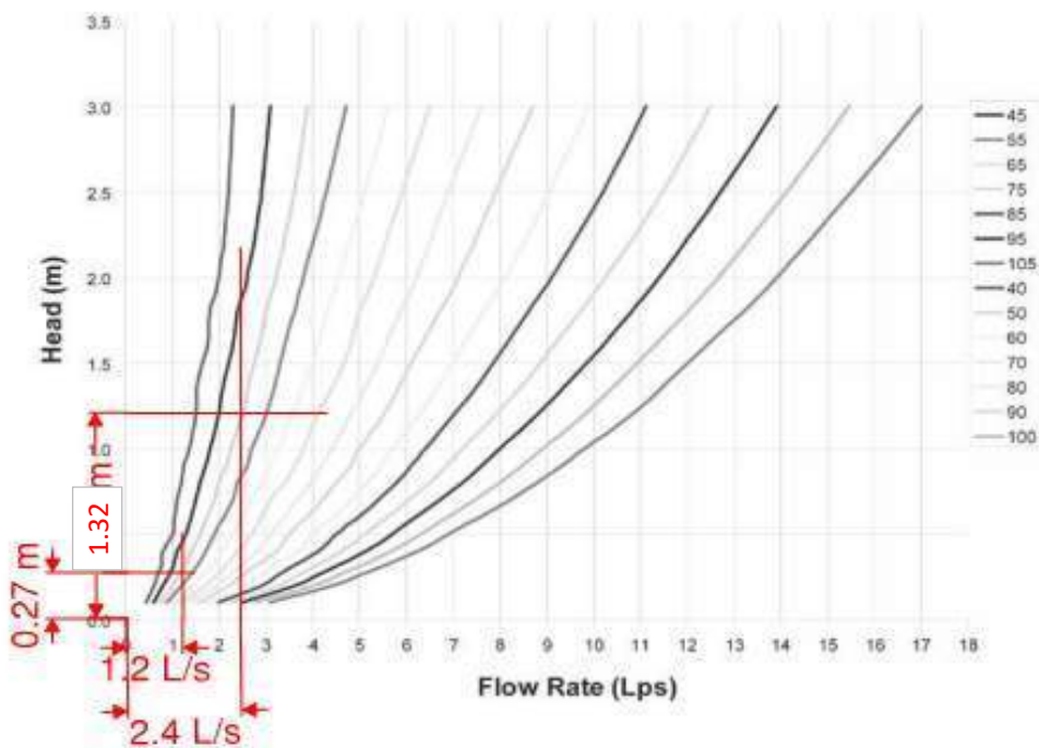
Chart 1: LMF 14 Preset Flow Curves
