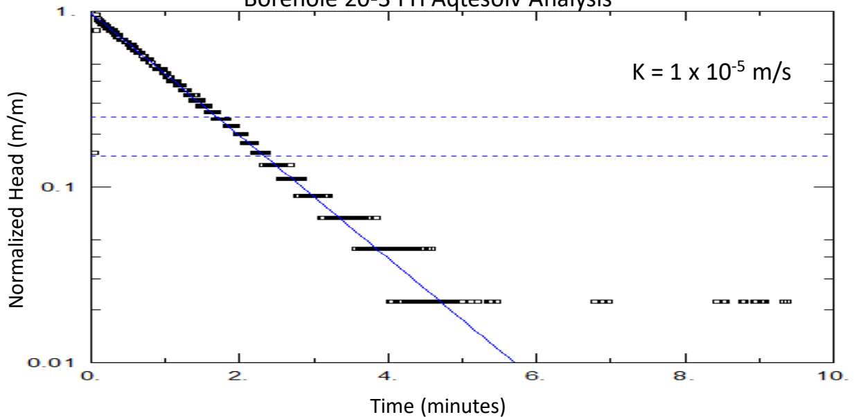
Borehole 20-3 FH Aquifer Analysis
