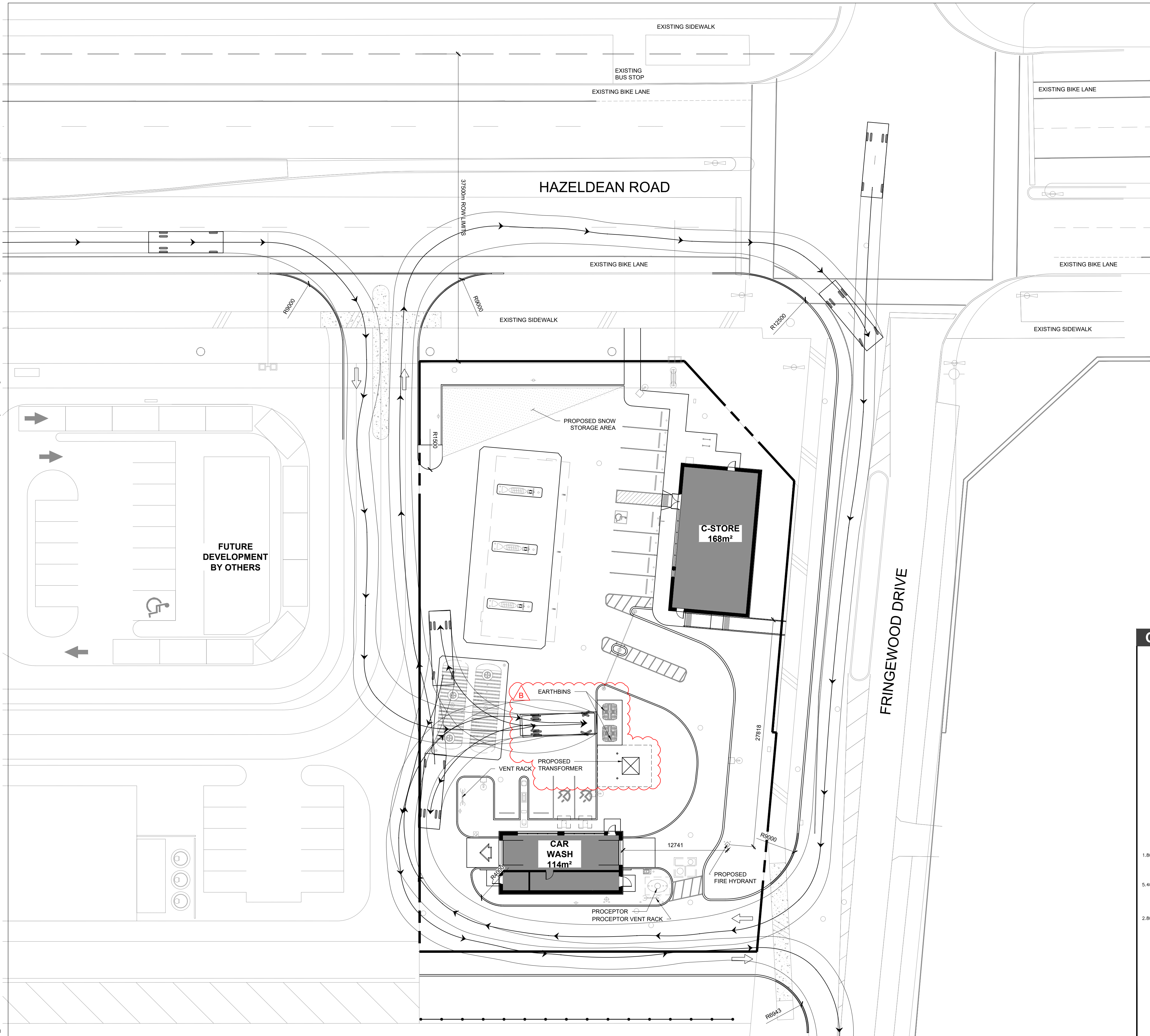
1 TRUCK ACCESS PLAN C111.0 SCALE: 1:250
