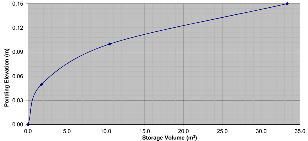
Stage Storage Curve: Area R-1 Controlled Roof Drain #11
