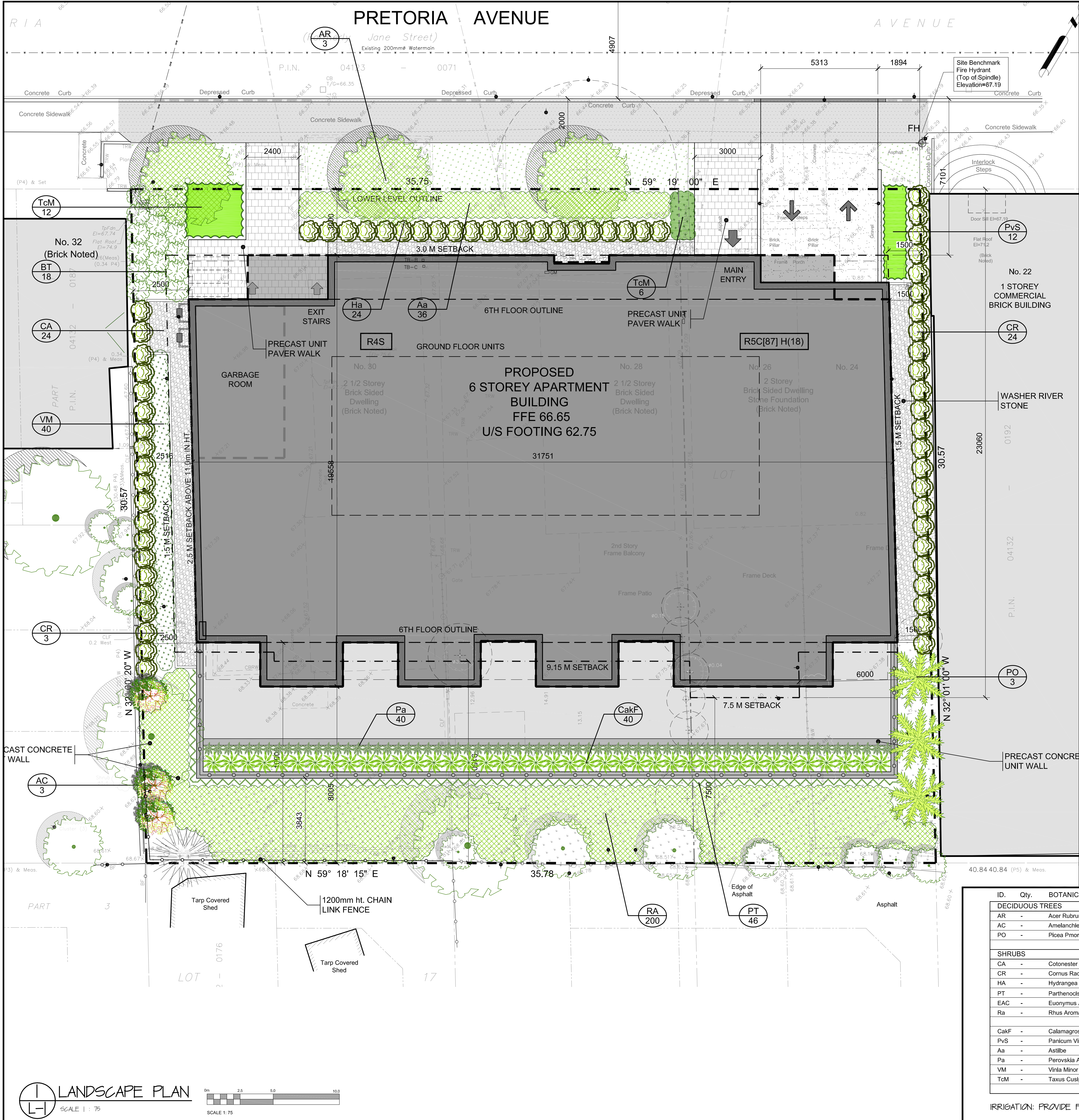
1. LANDSCAPE PLAN SCALE 1 : 75
