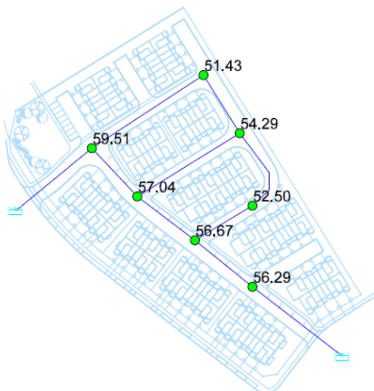
Figure 5 MXDY + 16,000L/min Fire Flow Results (Residual Pressure (psi))
