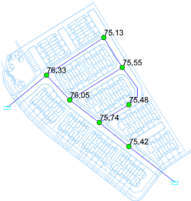
Figure 4 PKHR Pressure Results (psi)
