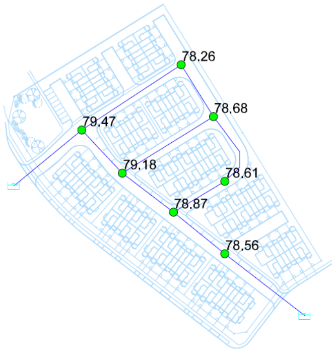
Figure 3 AVDY Pressure Results (psi)
