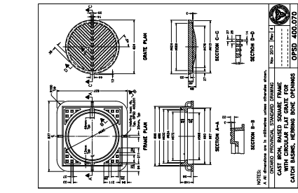
METHOD OF TERMINATION FOR CURB WITH CIRCULAR FLAT GRATE FOR CATCH BASINS, HEBLING BONE SYSTEMS OPSP 400.070
