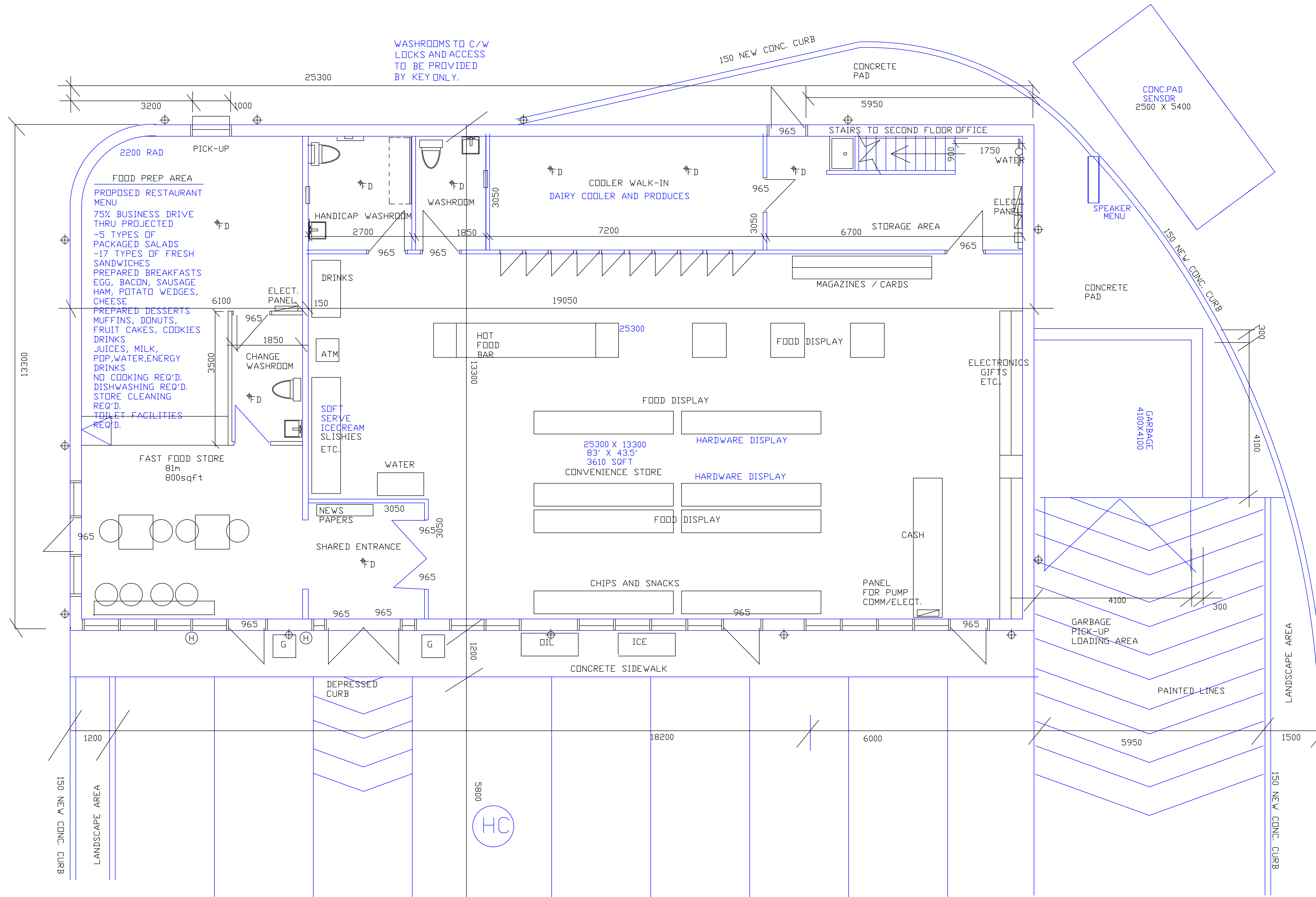
FURNITURE EQUIPMENT PLAN
