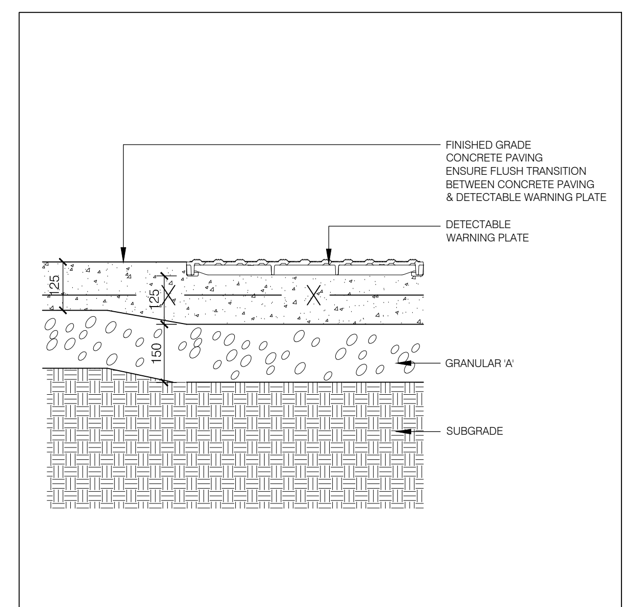
D3 DETECTABLE WARNING STRIP L101 SECTION SCALE 1:10
