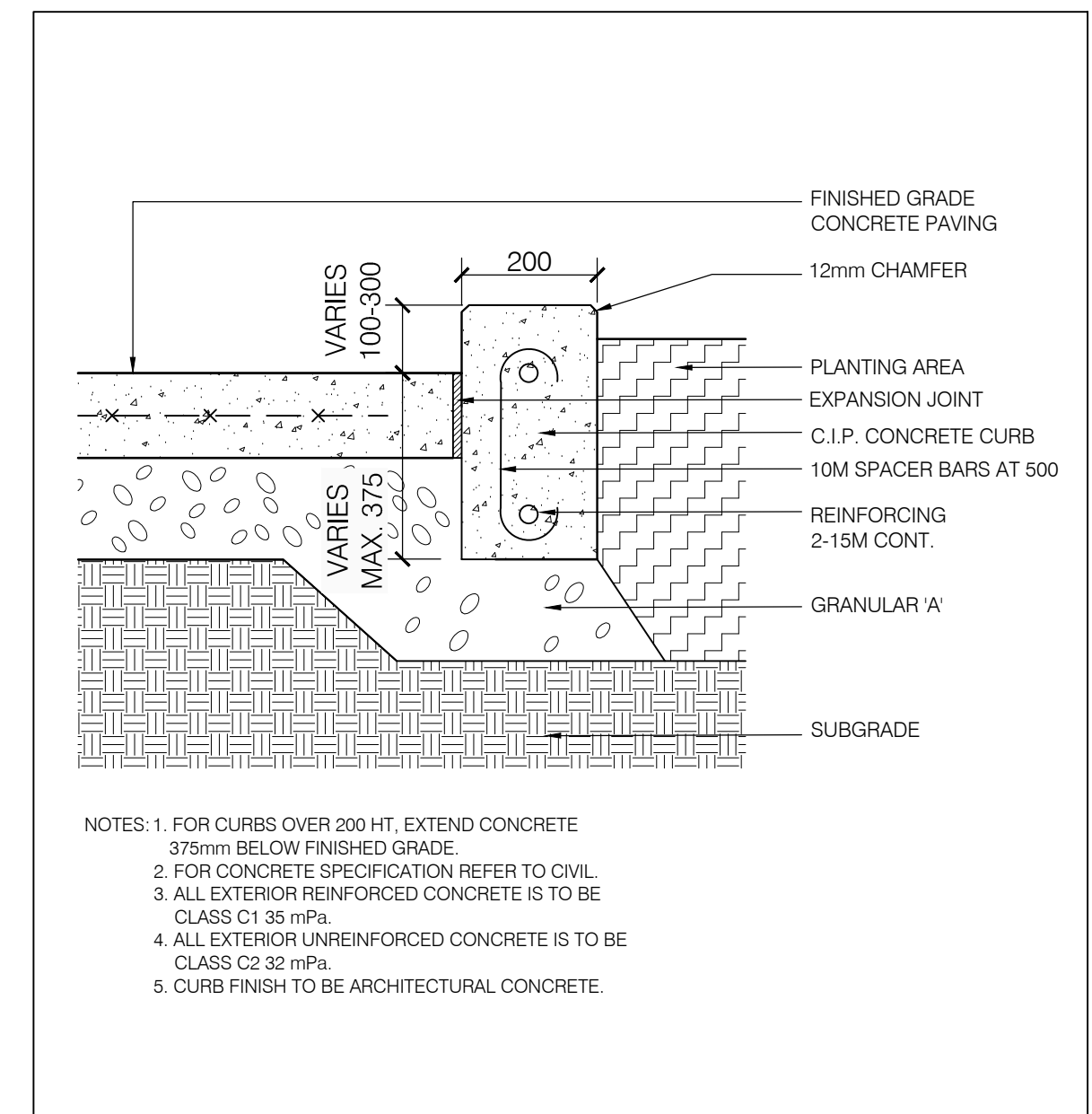
D2 TYPICAL CONCRETE PLANTER CURB ON GRADE L101 SECTION SCALE 1:10
