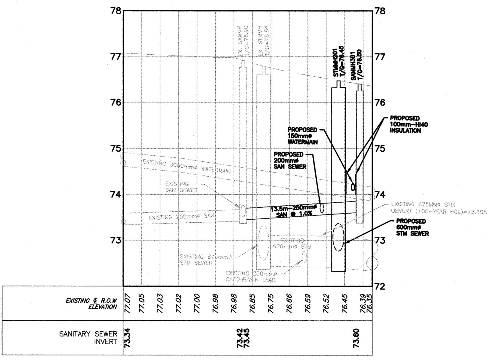
SANDHILL ROAD SANITARY EXTENSION SCALE: HORIZ 1:250 VERT 1:50
