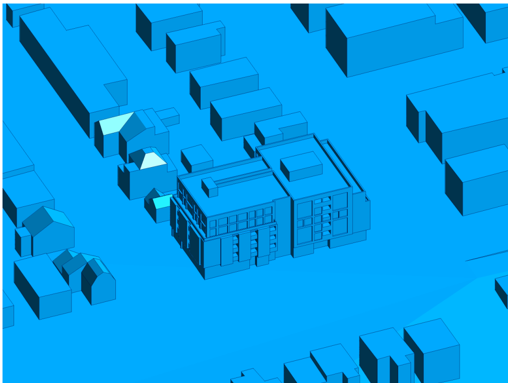
FIGURE 2B: STUDY BUILDING, NORTH PERSPECTIVE
