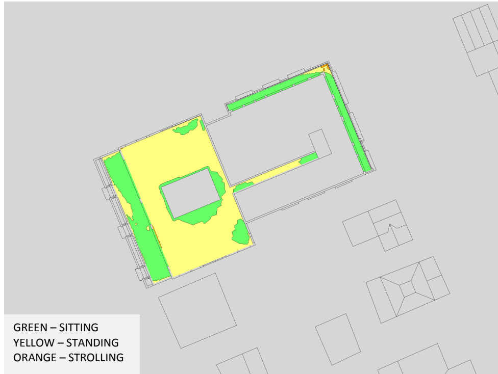
FIGURE 3B: SPRING – TERRACE WIND CONDITIONS
