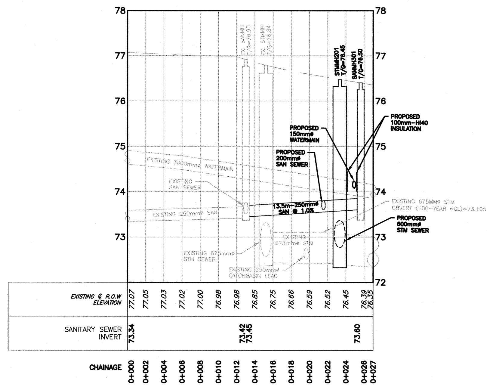
SANDHILL ROAD SANITARY EXTENSION SCALE: HORIZ 1:250 VERT 1:50
