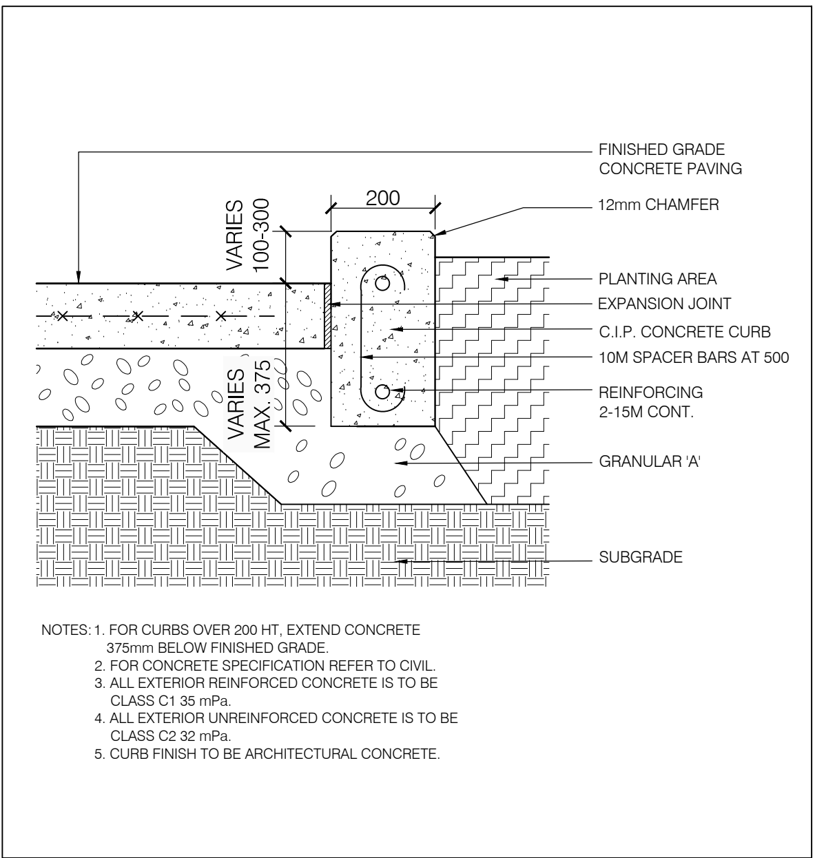
D2 L101 TYPICAL CONCRETE PLANTER CURB ON GRADE SECTION SCALE 1:10
