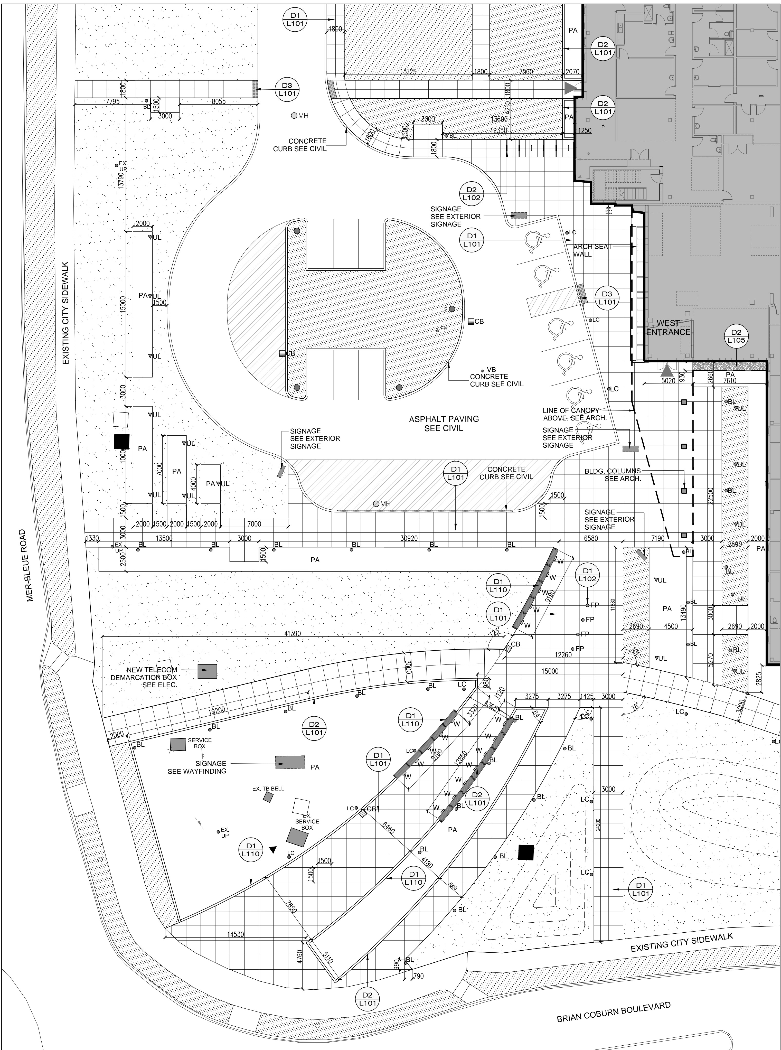
L1 L101 WEST ENTRANCE LAYOUT PLAN PLAN SCALE 1:200
