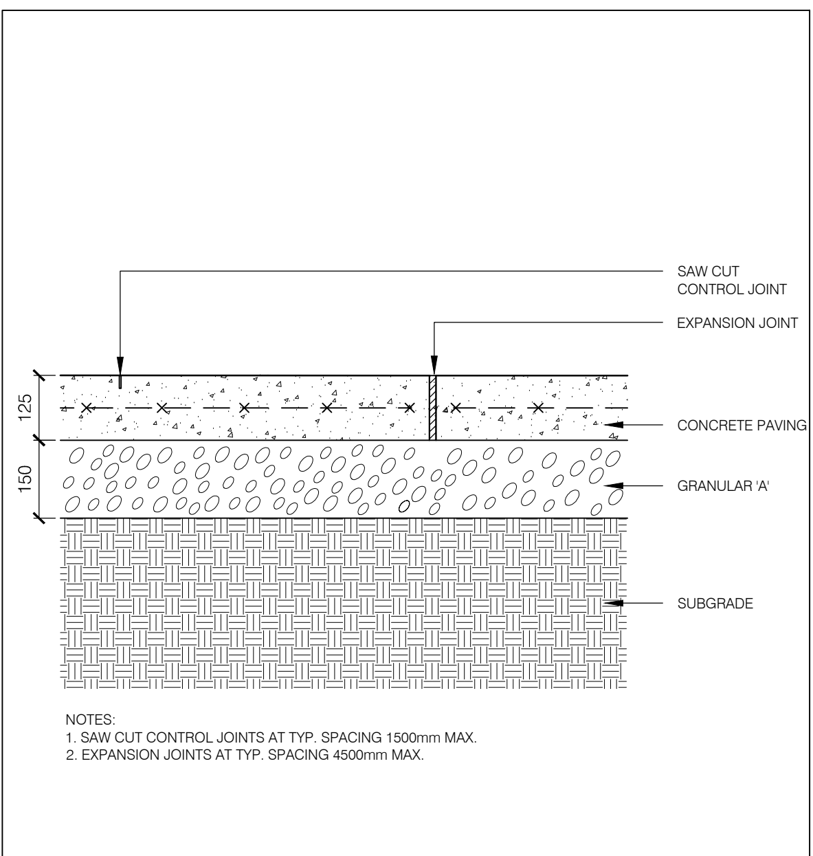
D1 L101 TYPICAL CONCRETE PAVING ON GRADE SECTION SCALE 1:10
