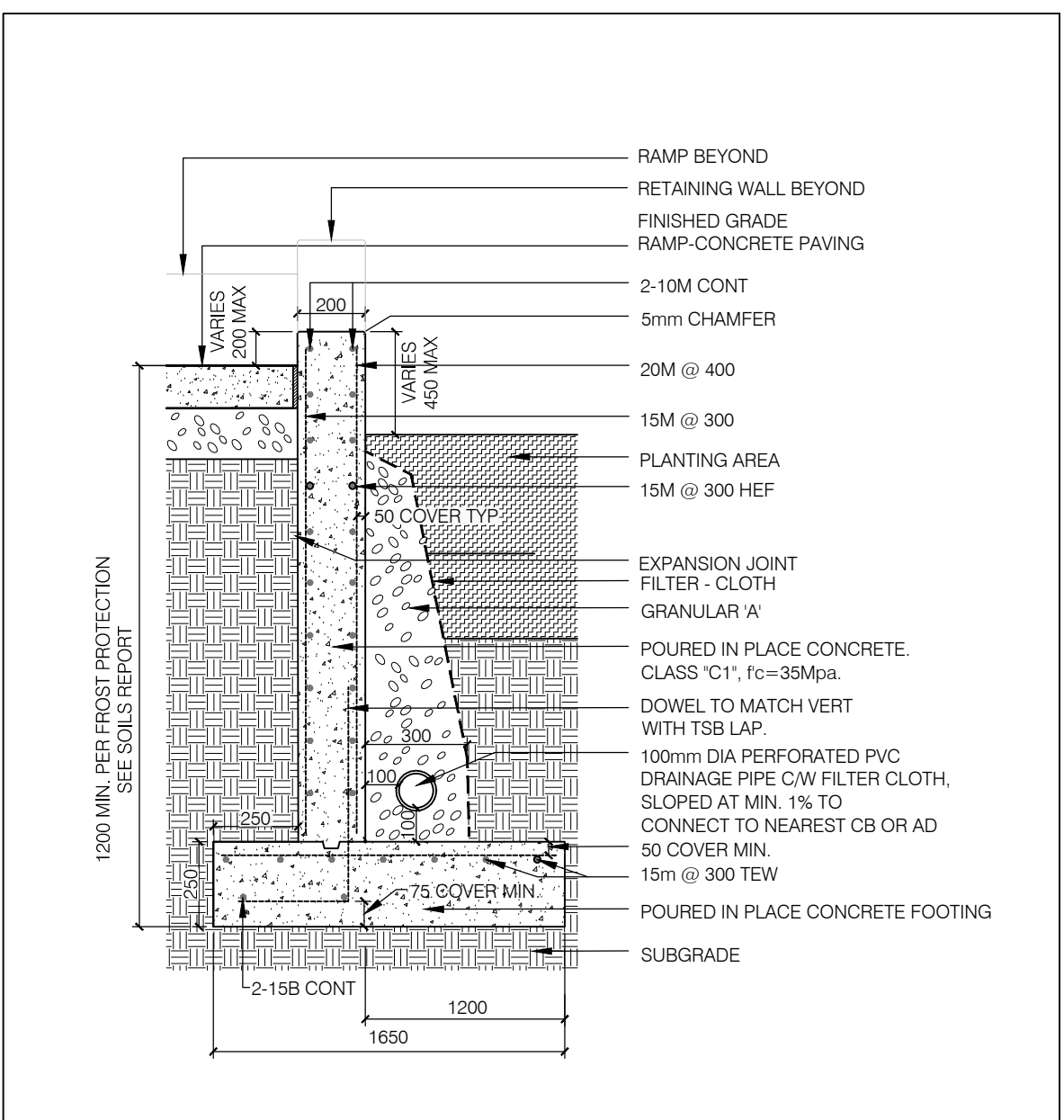
D4 L101 TYPICAL CONCRETE PLANTER RETAINING WALL SECTION SCALE 1:10
