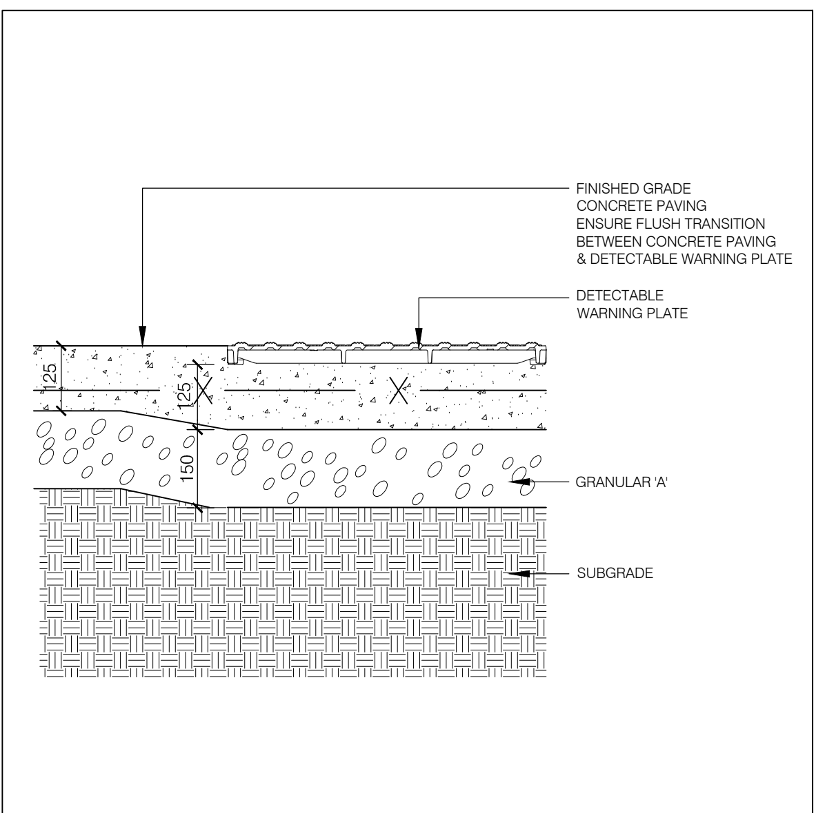
D3 L101 DETECTABLE WARNING STRIP SECTION SCALE 1:10
