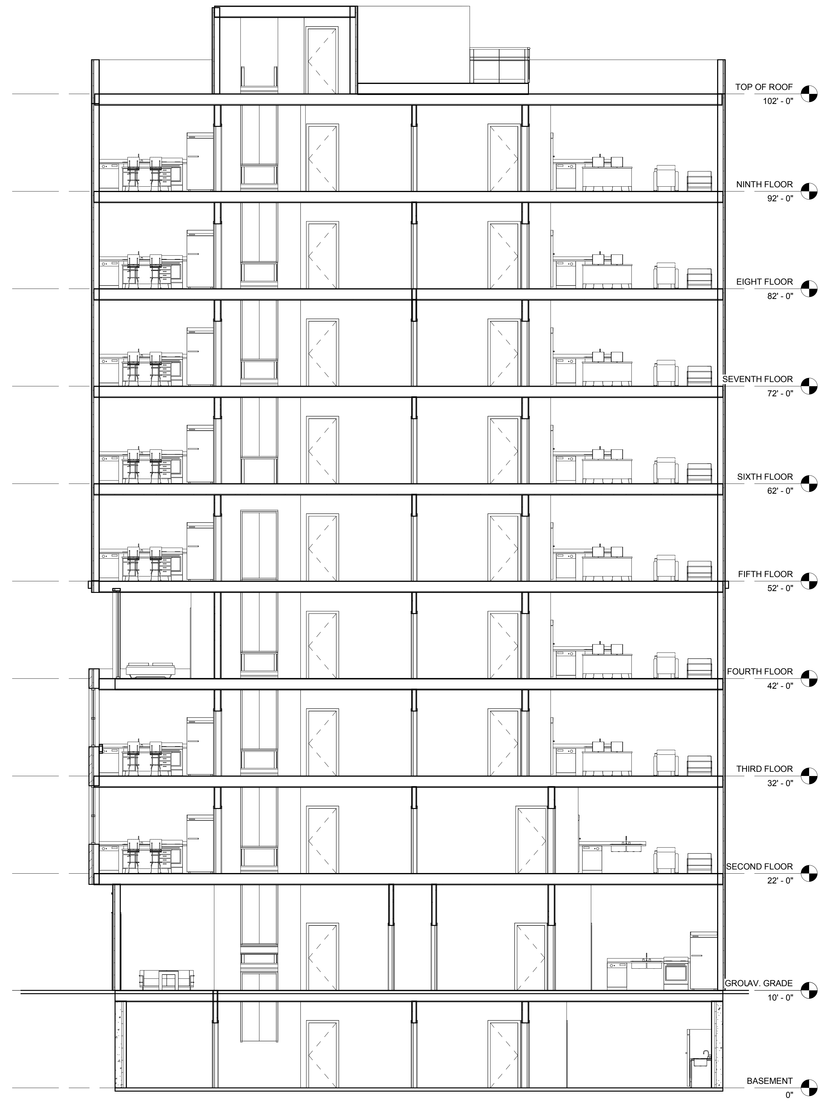
1 Section 1 3/16" = 1'-0"
