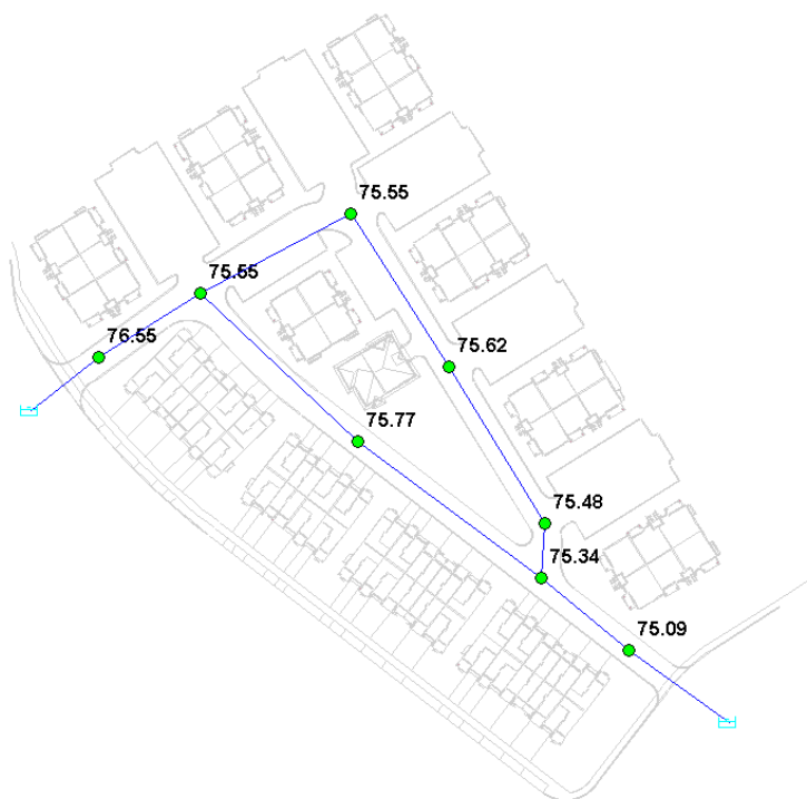
Figure 4 PKHR Pressure Results (psi)
