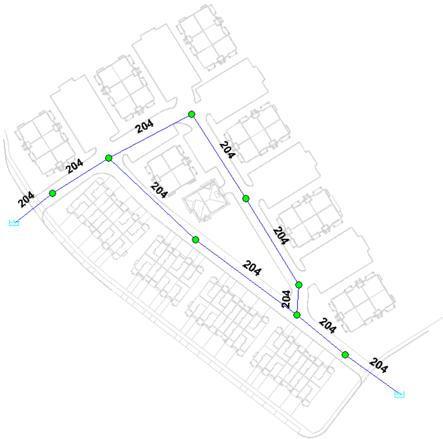
Figure 2 Proposed Watermain Layout
