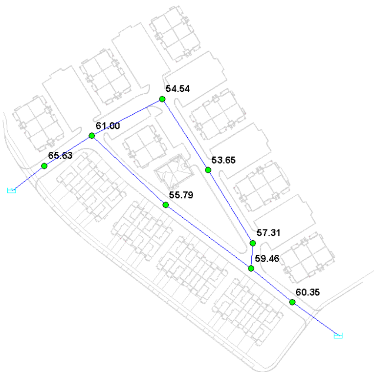
Figure 5 MXDY + 15,000L/min Fire Flow Results (Residual Pressure (psi))
