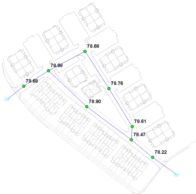
Figure 3 AVDY Pressure Results (psi)
