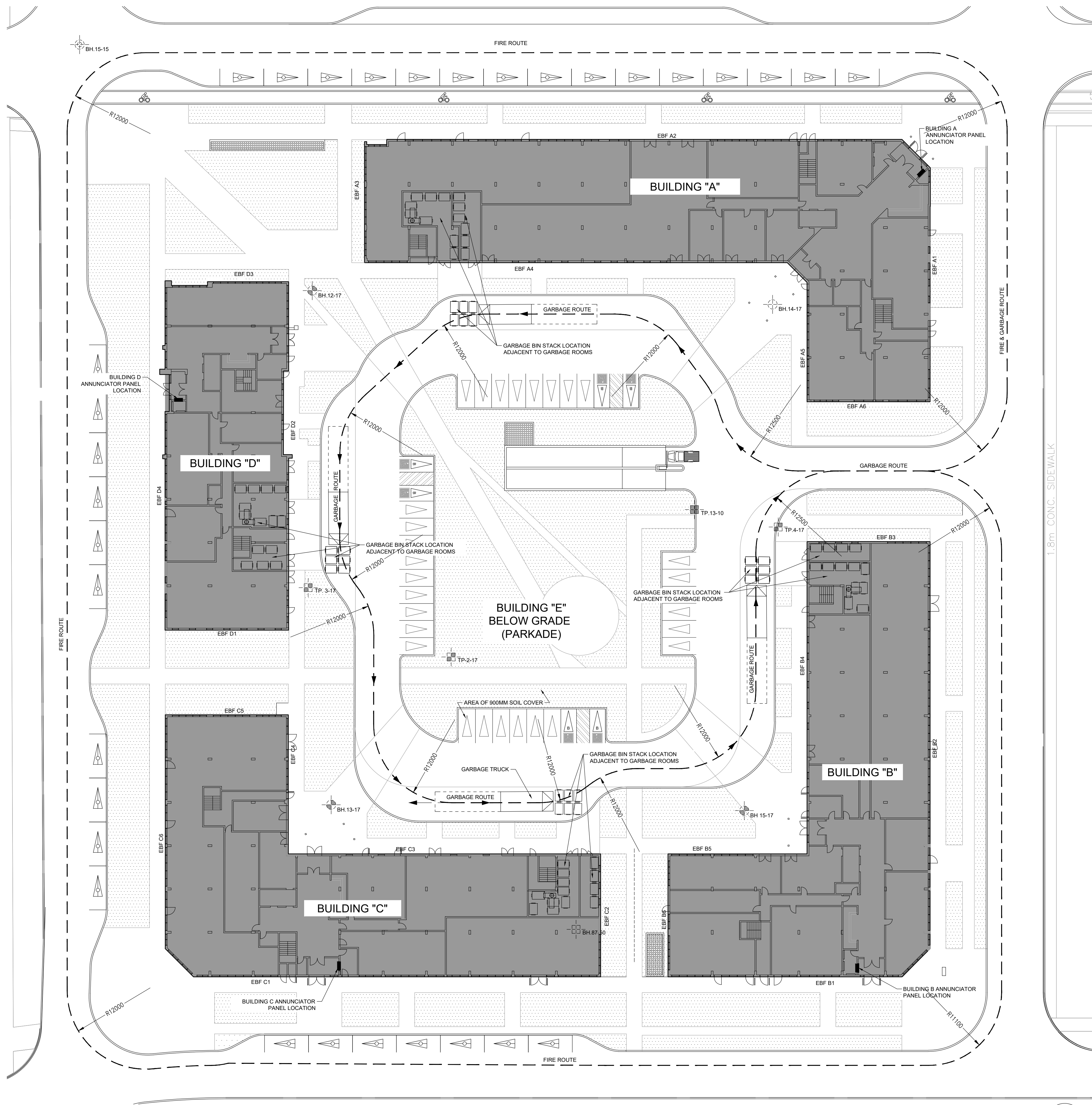
SITE DETAILS - FIRE & GARBAGE ROUTES 1 1:250 102
