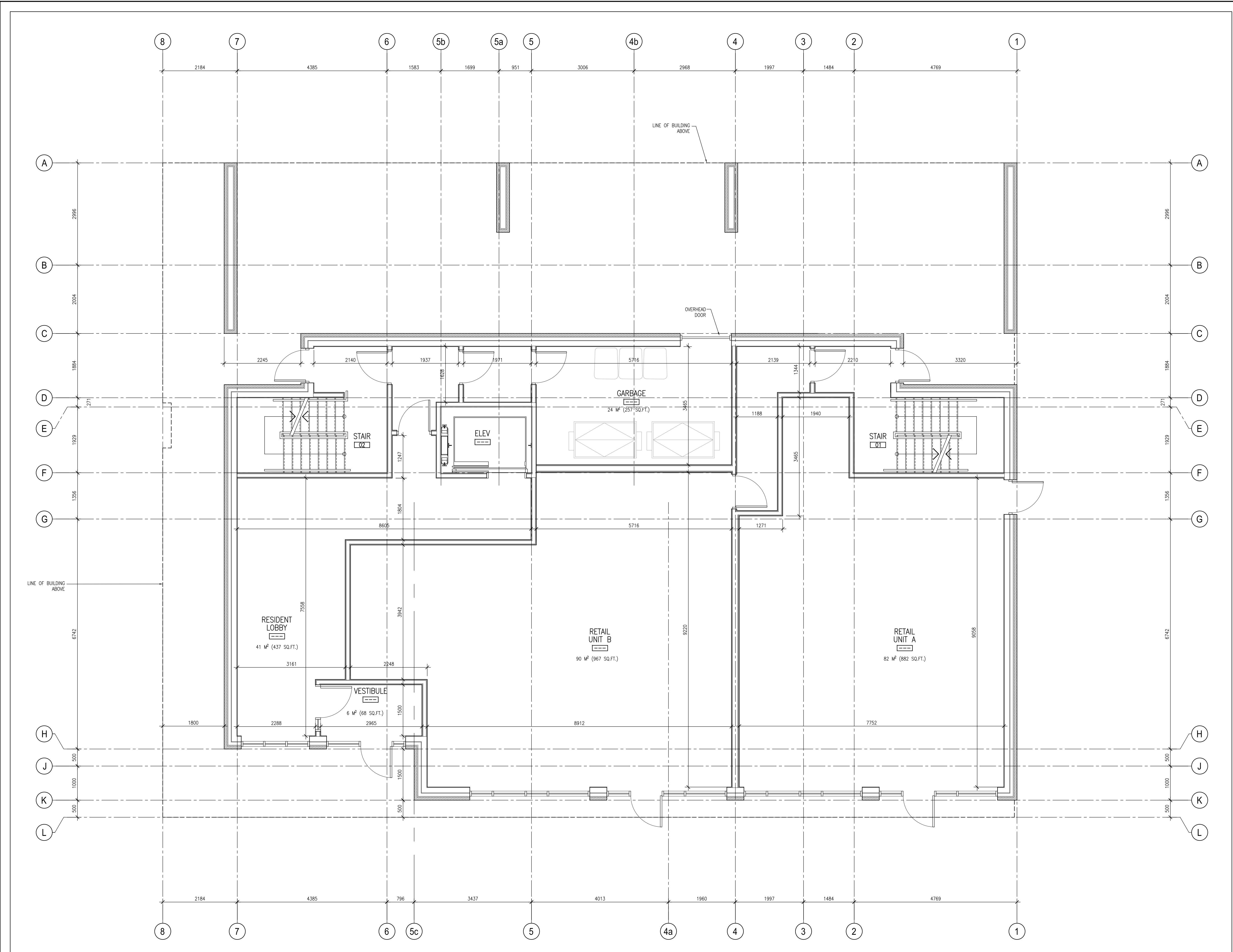
1 LEVEL 01 FLOOR PLAN A101 SCALE: 1:50
