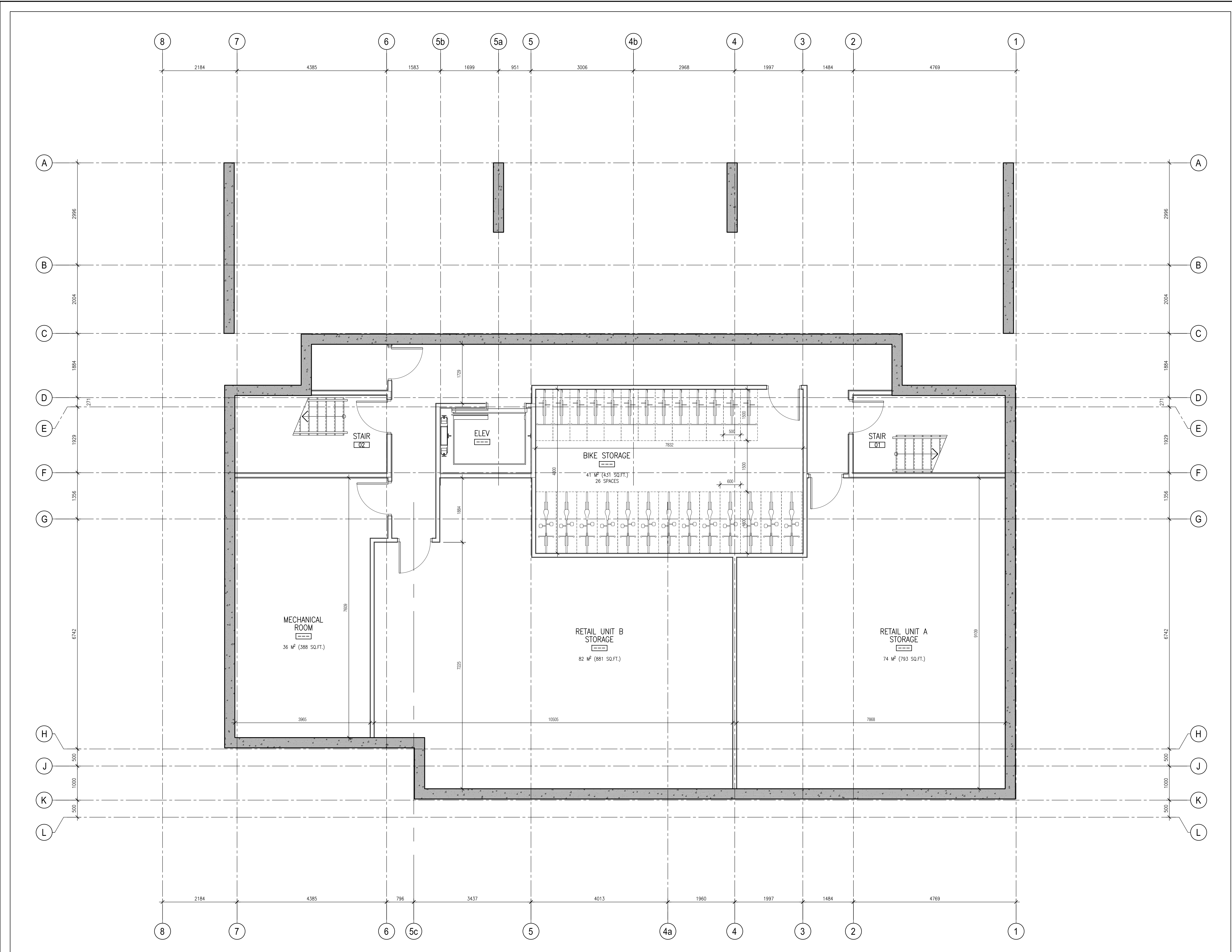
1 LEVEL 00 FLOOR PLAN A100 SCALE: 1:50
