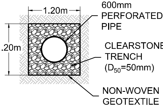
DETAIL: INFILTRATION TRENCH CROSS-SECTION SCALE: 1:50
