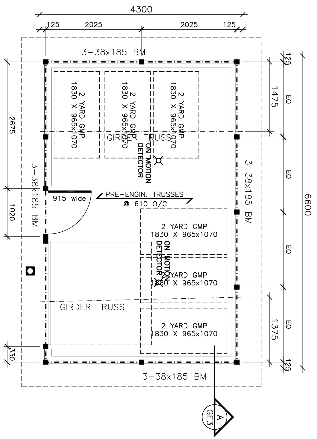
FLOOR PLAN
