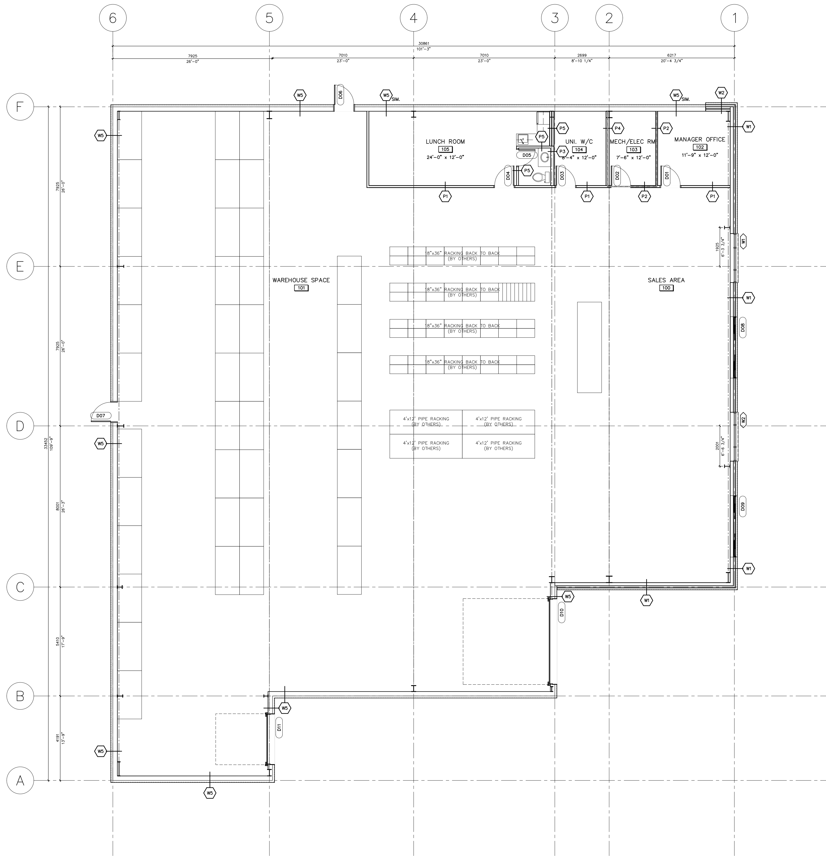
01 GROUND FLOOR PLAN A201 SCALE: 1: 96 1/8" = 1'-0"
