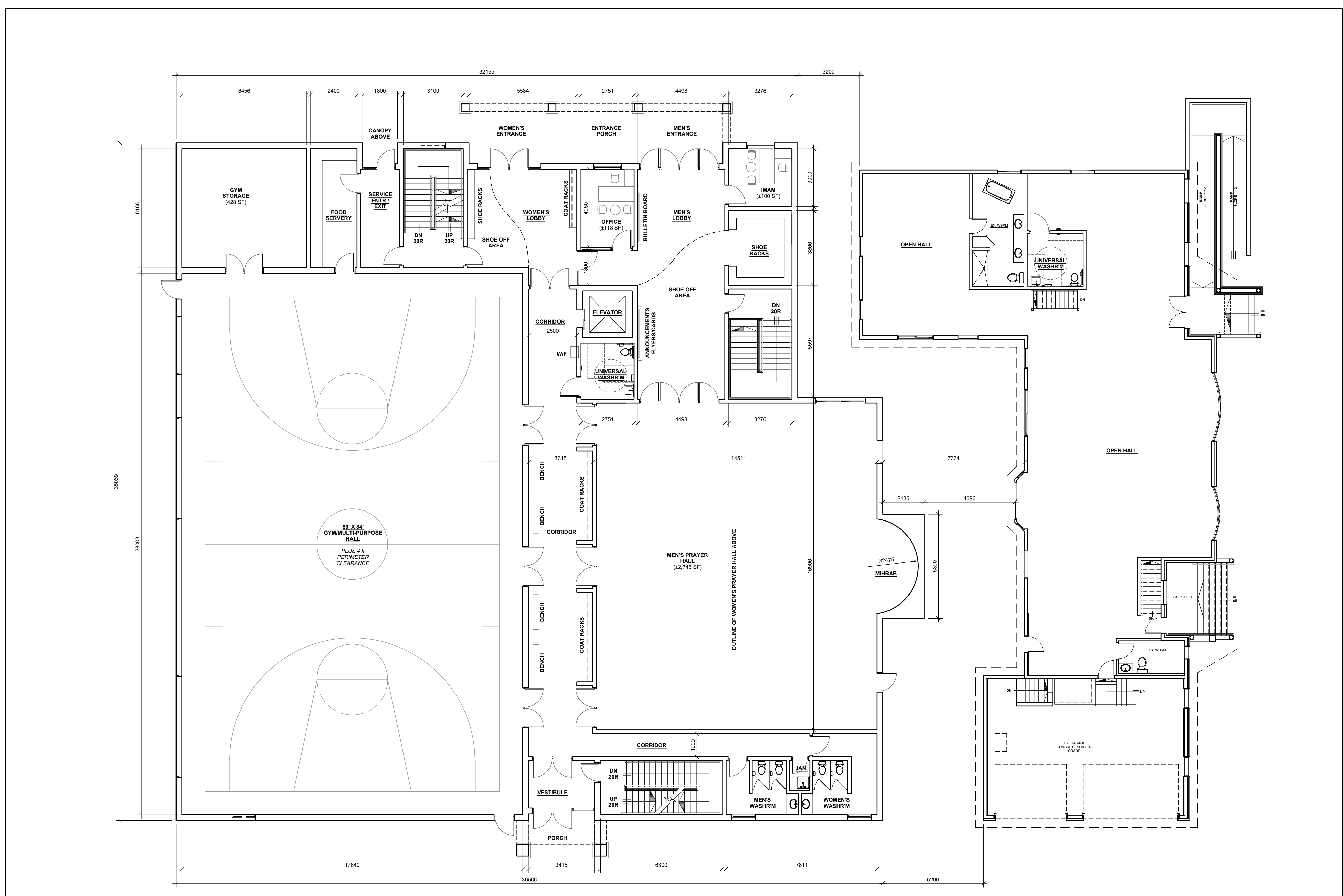
1 PROPOSED FIRST FLOOR PLAN - PHASE (2) A2.0 SCALE 1:100
