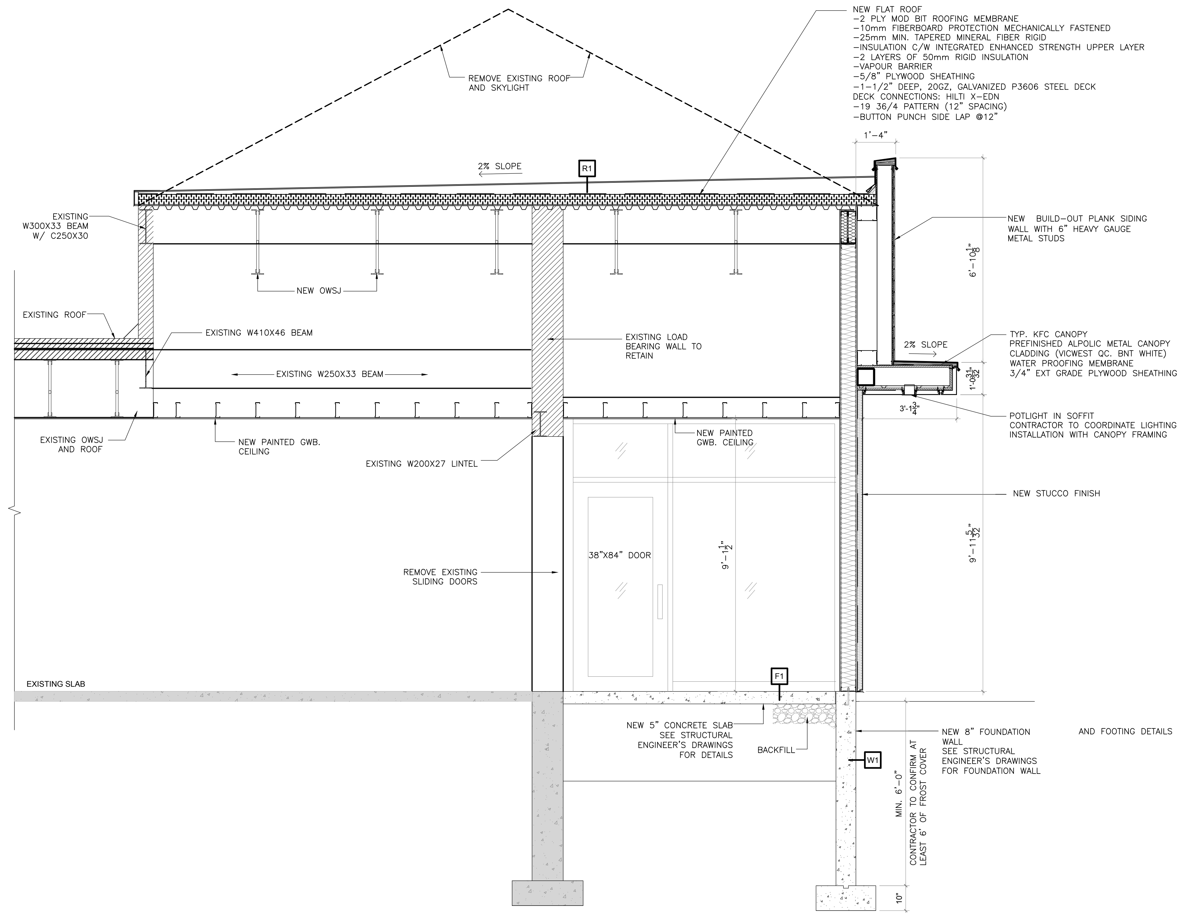
1 A.6 BUILDING SECTION THROUGH ENTRANCE 1/2"=1'
