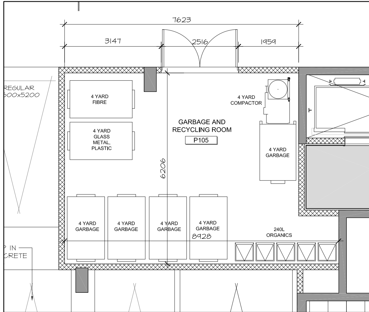
GARAGE P1- GARBAGE/ RECYCL ROOM
